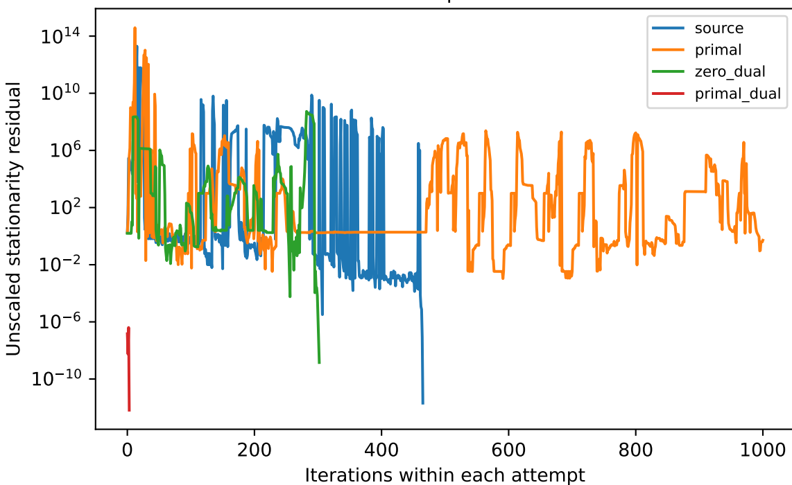
IEEE 300 | load 1.0
