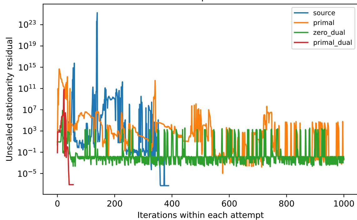
IEEE 300 | load 1.0
