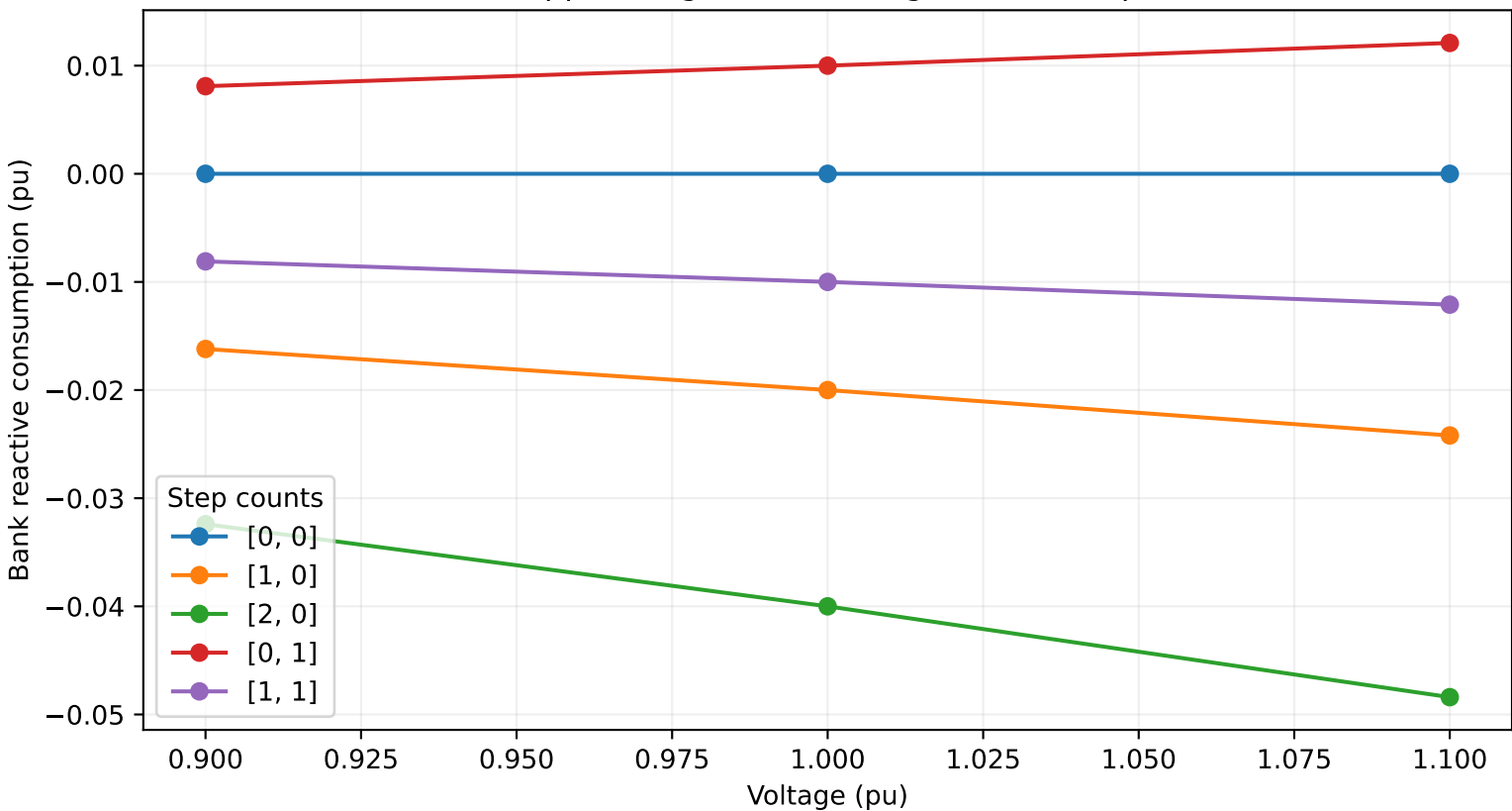
M6.2: supplied legal states · negative Q is capacitive
