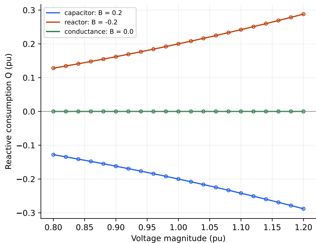
M6.1 · Fixed shunts: analytic lines and computed markers
