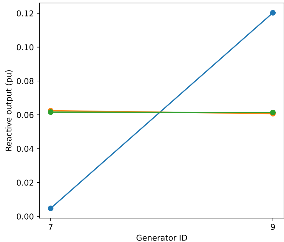
Matched fixed / optimized tap configurations
