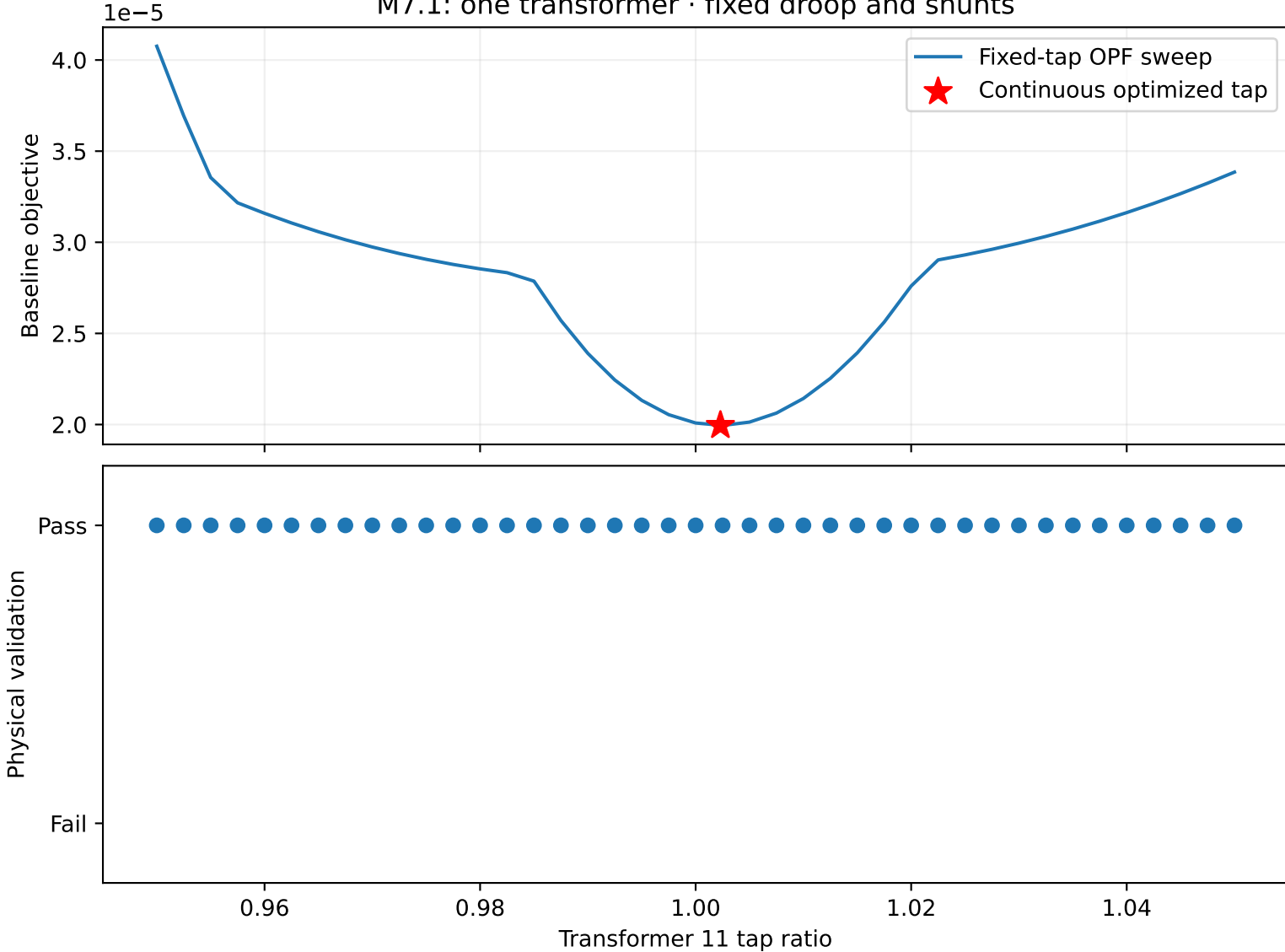
M7.1: one transformer · fixed droop and shunts
