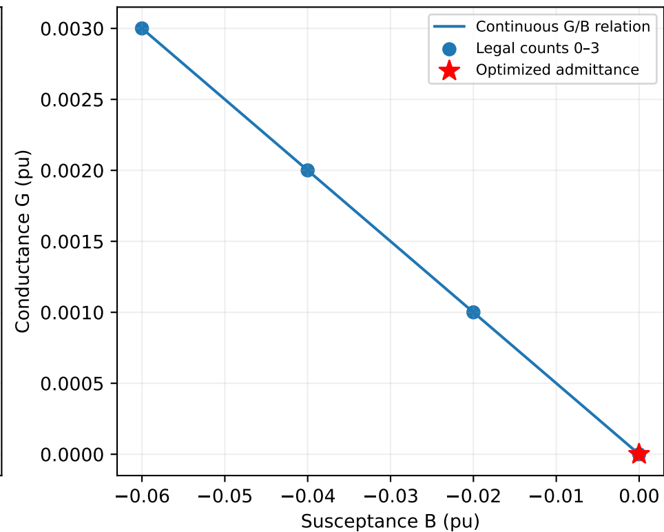
reactor
