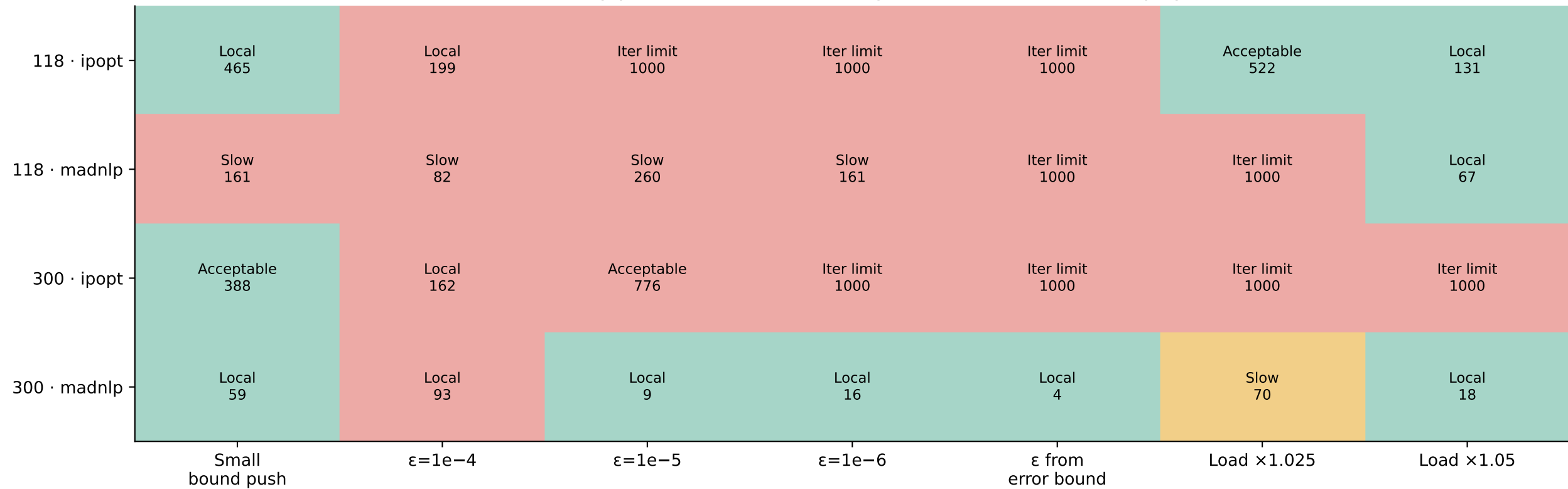
Recovery probes · coarse smoothing is allowed to fail exact replay
