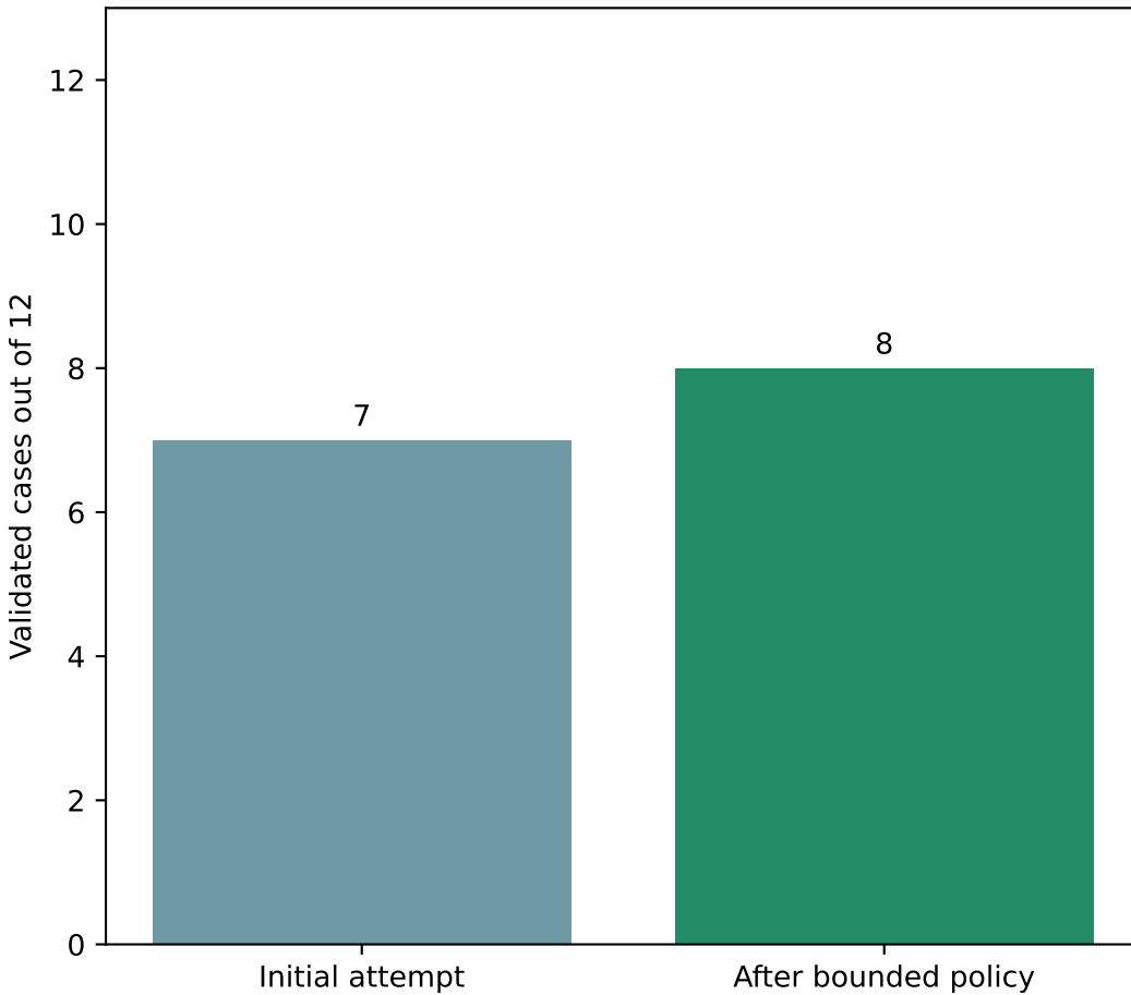
ipopt
