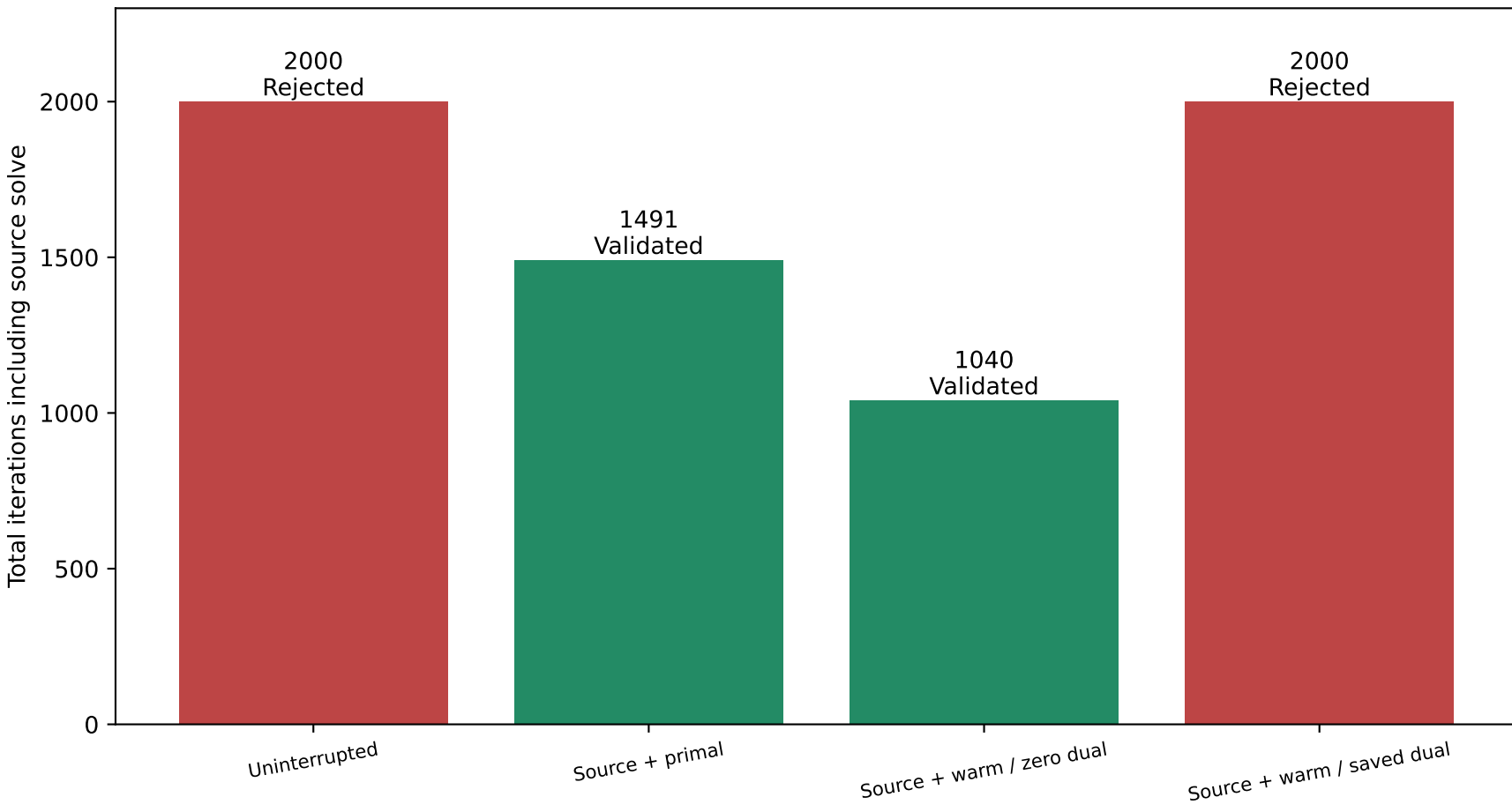
Stressed IEEE 300: equal total budget of 2000 iterations / 120 CPU seconds
