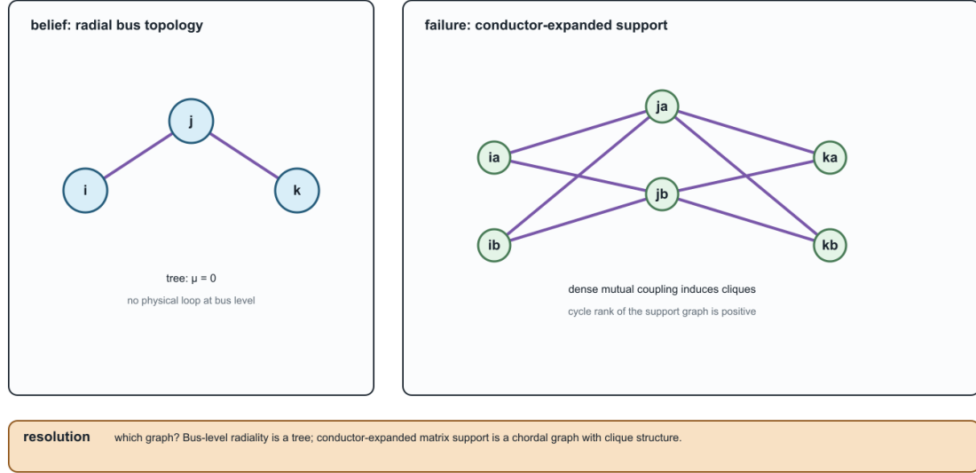
Figure 5.1: A radial bus-level feeder can have cycles in its conductor-expanded support graph.
