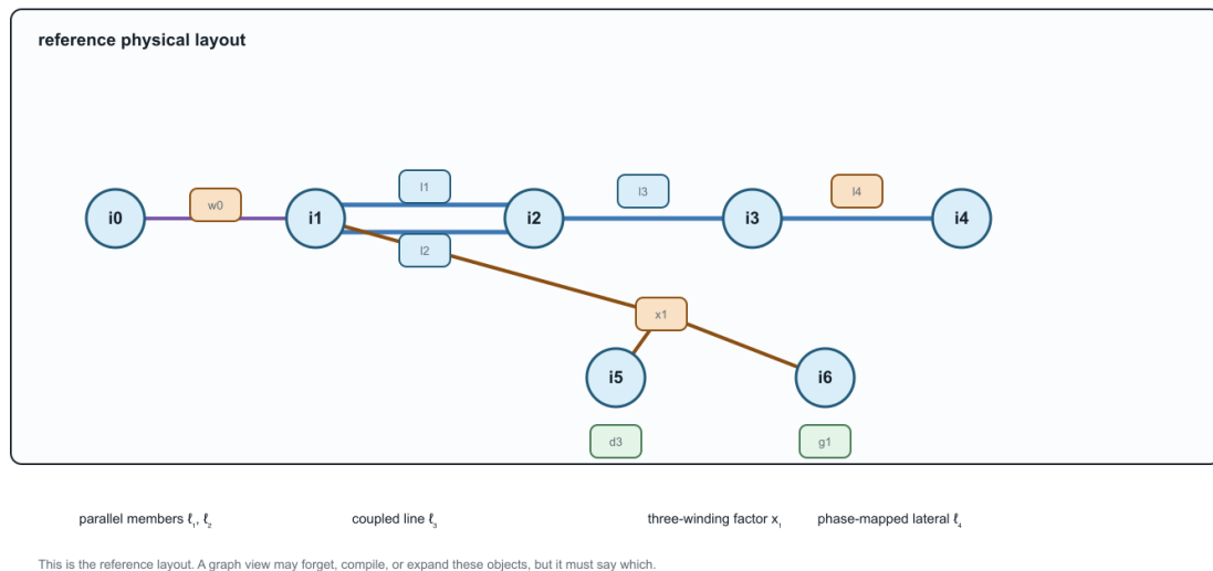
Figure 26.1: Reusable physical layout of the running multiconductor network.
