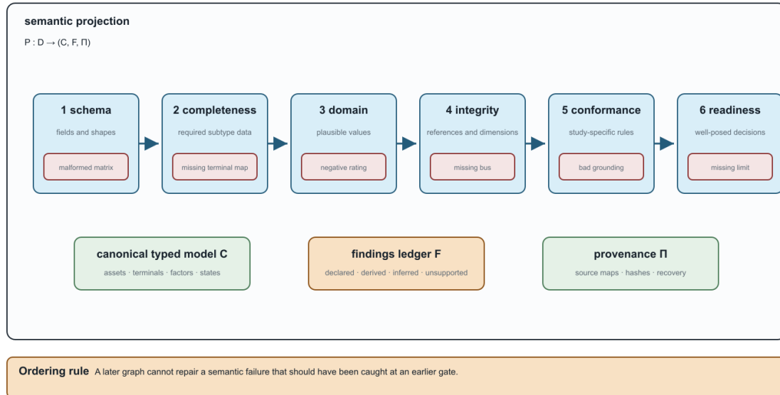
Figure 20.1: The ordered source-to-canonical validation pipeline.
