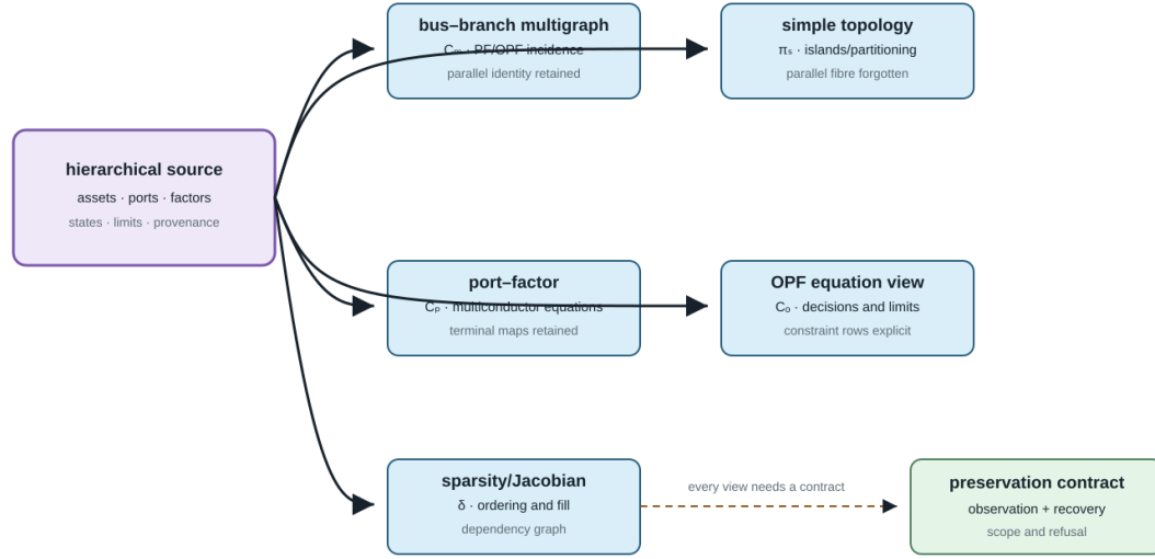
Figure 13.1: One source architecture feeding several typed maps.
