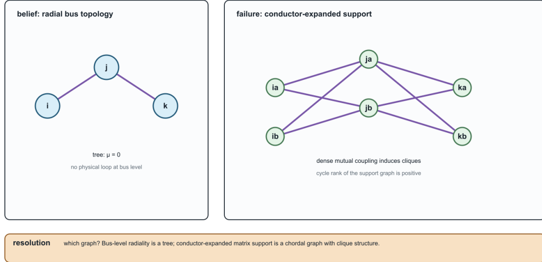
Figure 3.1: A radial bus-level feeder can have cycles in its conductor-expanded support graph.
