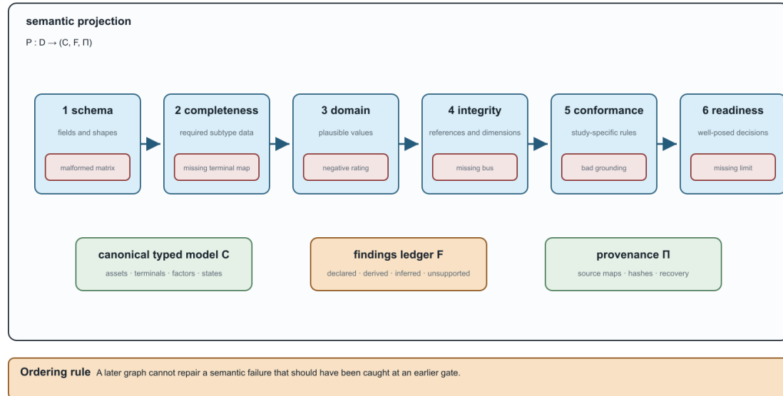
Figure 21.1: The ordered source-to-canonical validation pipeline.
