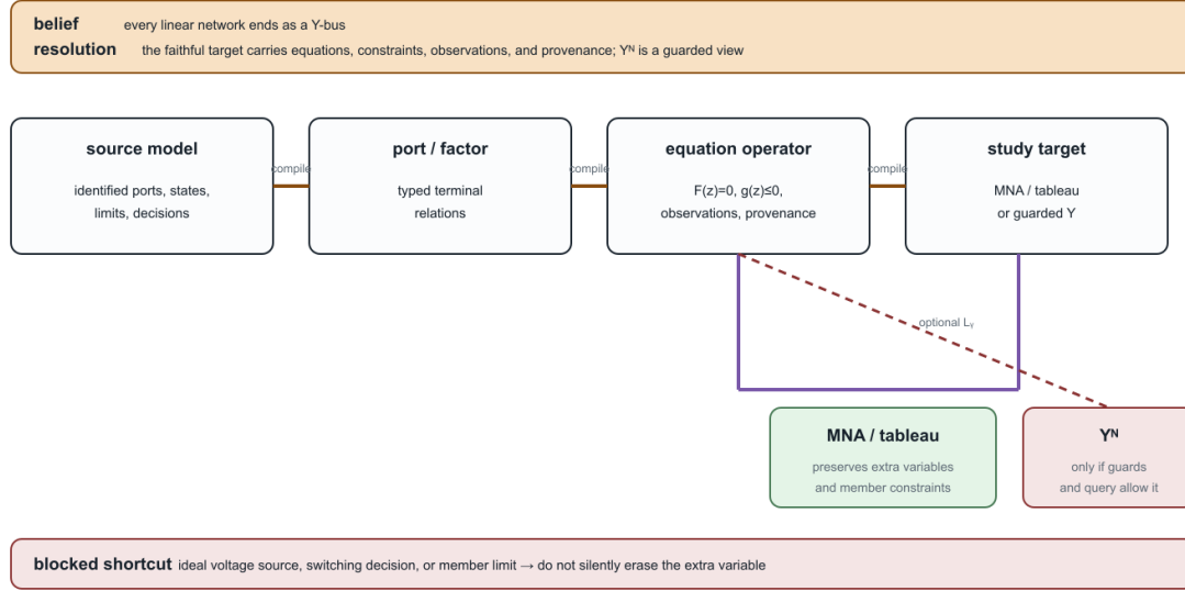
Figure 18.3: The formulation-lowering lattice: the equation/constraint operator is the faithful boundary, while MNA/tableau and nodal admittance are guarded study targets.
