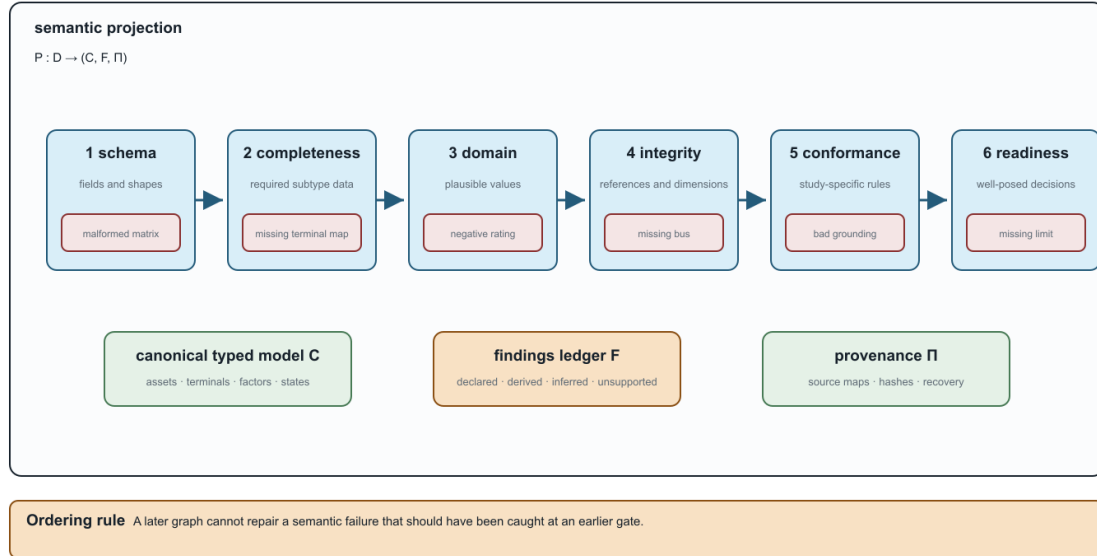
Figure 20.1: The ordered source-to-canonical validation pipeline.
