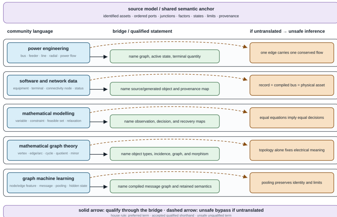
Figure 5.1: Five communities approach the book's shared semantic anchor through different vocabularies; a dashed bypass shows the unsafe inference made when the bridge is skipped.
