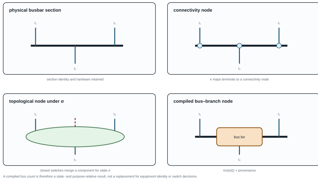
Figure 26.2: One substation shown as four bus representations.
