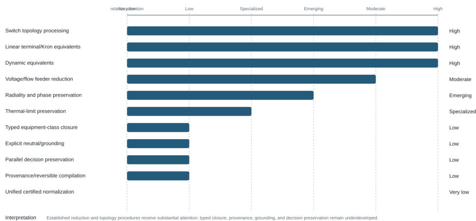
Figure 52.1: Provisional literature attention and structured gaps across the preservation agenda.
