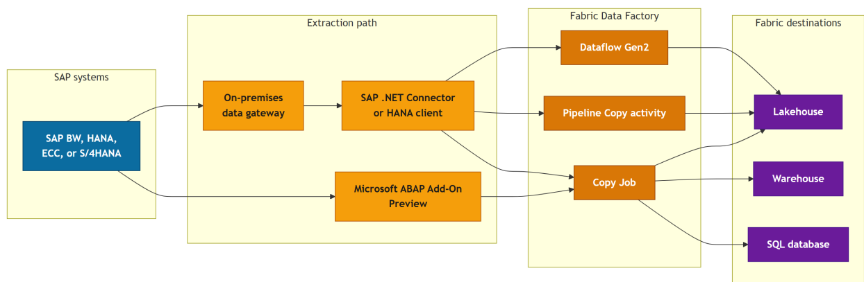
Figure 3: Architecture 2
