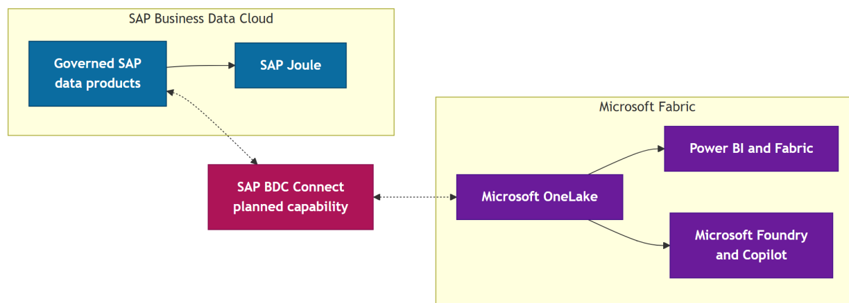
Figure 10: Architecture 9
