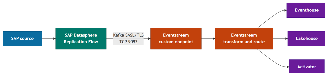
Figure 8: Architecture 7
