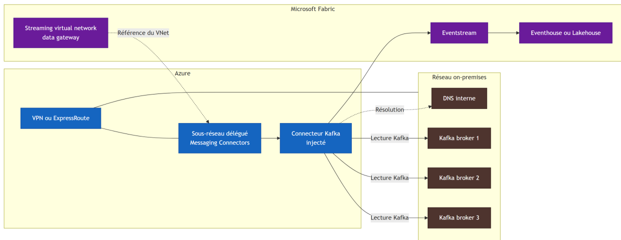
Figure 2: Architecture 2
