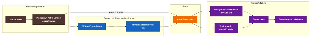
Figure 3: Architecture 3
