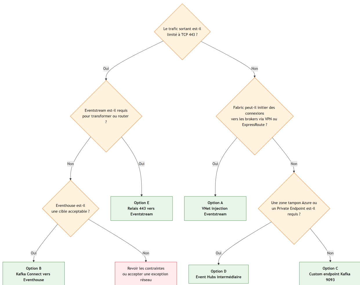
Figure 4: Architecture 4
