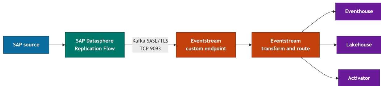
Figure 8: Architecture 7
