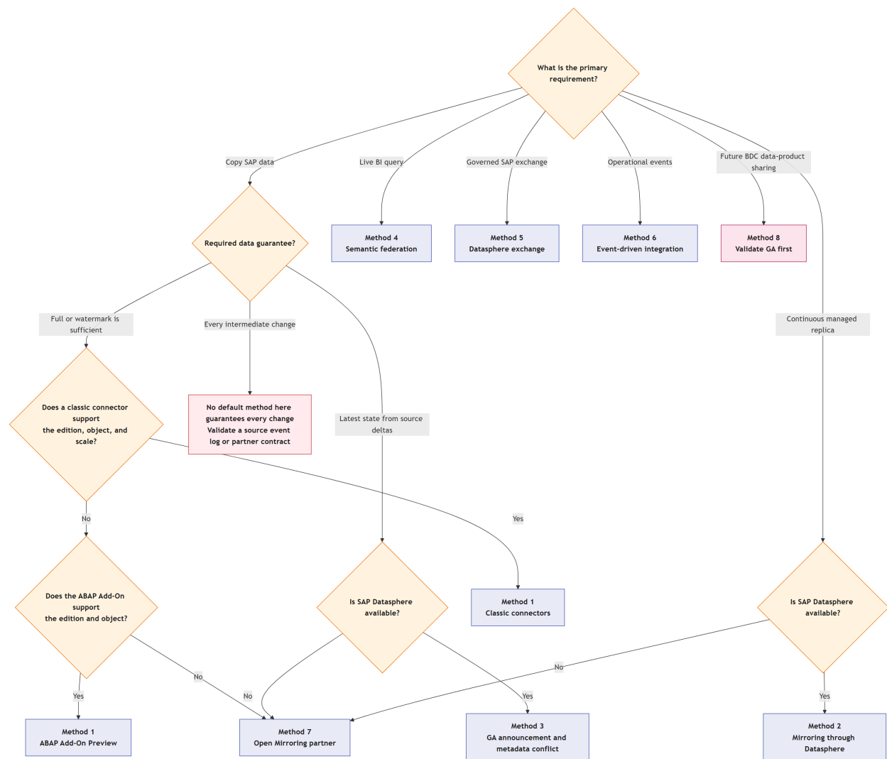
Figure 11: Architecture 10
