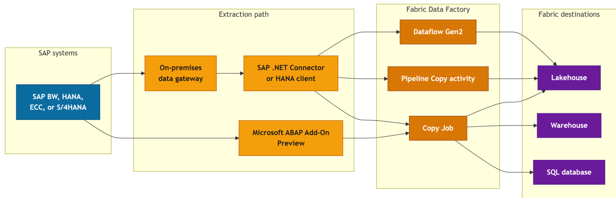
Figure 3: Architecture 2
