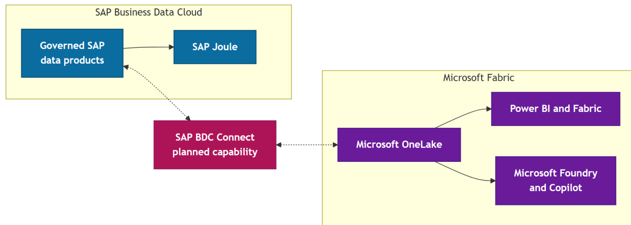
Figure 10: Architecture 9
