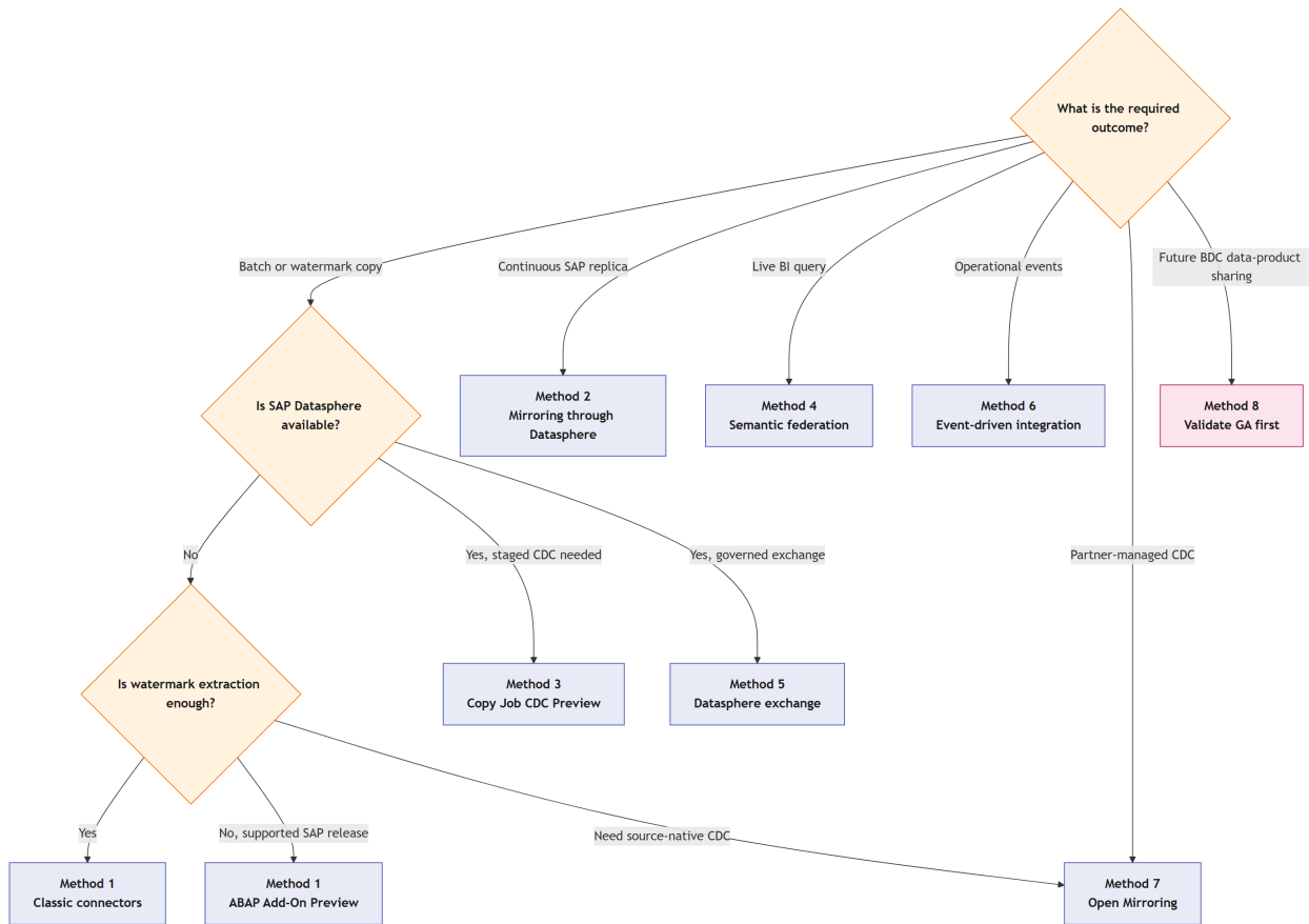
Figure 11: Architecture 10
