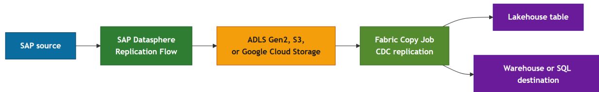
Figure 5: Architecture 4
