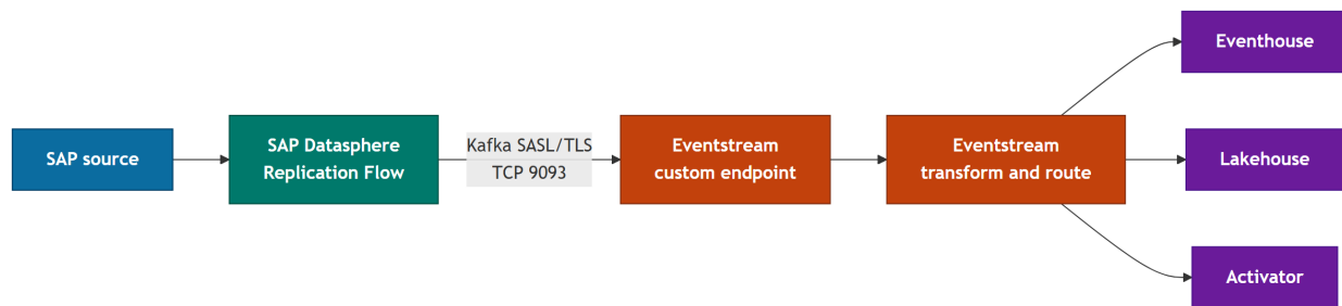
Figure 8: Architecture 7
