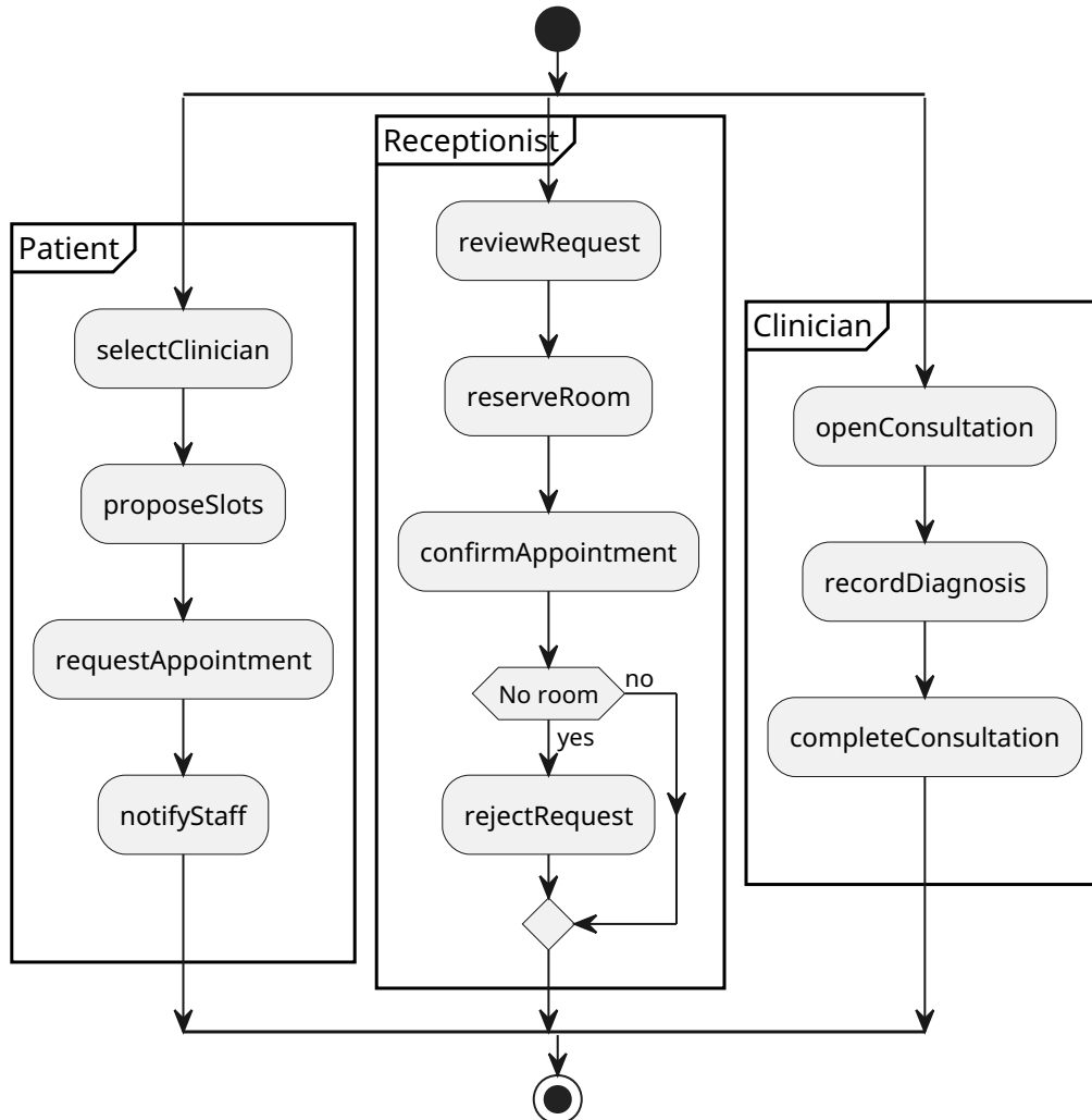
Activity Diagram: Clinic Scheduling System
