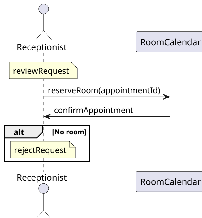
Sequence Diagram: ConfirmAppointment
