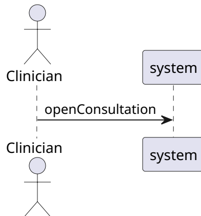
System Sequence Diagram: CompleteConsultation
