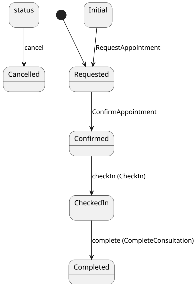
State Machine: Appointment
