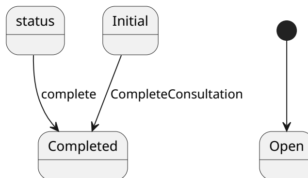
State Machine: Consultation
