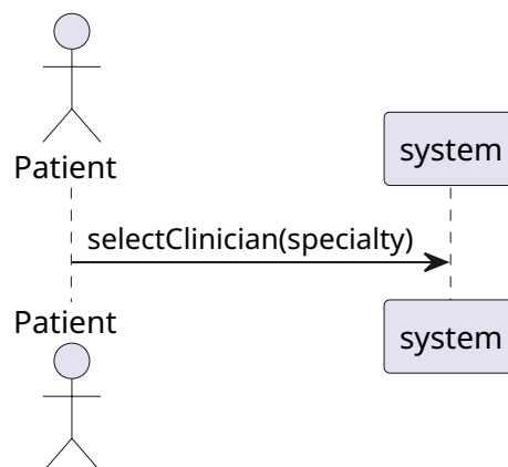
System Sequence Diagram: RequestAppointment
