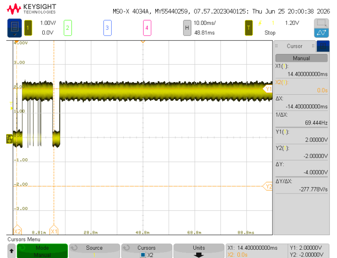
Fig. 17. Capture of the receiver data output during initial code acquisition. The transmitted data bit is fixed to “1”. During code acquisition, the receiver attempts to decode data from every candidate code offset as they are found, so random data is output until finally the correct code offset is acquired and locked onto.
