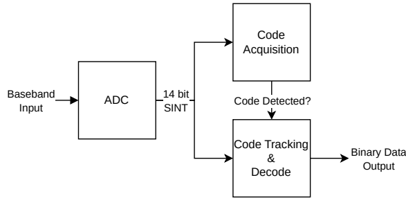
Fig. 3. Overview of the basic building blocks of the receiver. The analog baseband input gets sampled by the ADC. The code acquisition block finds the maximum correlation offset of a local code replica with the signal, at which point the tracking and decode block is enabled.
