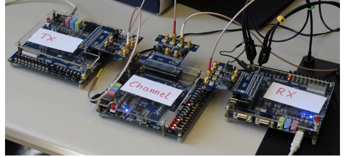
Fig. 5. Full Setup on Cyclone II FPGAs
