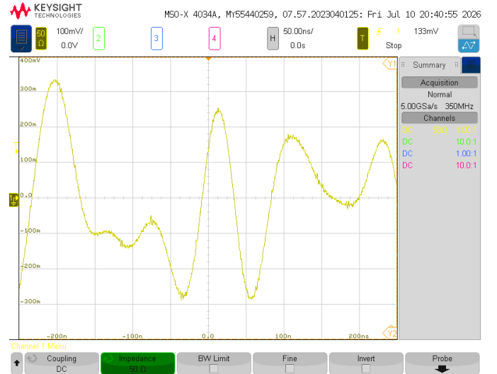
Fig. 12. Oscilloscope capture of the 11MHz low-pass filtered transmitter output signal.
