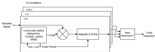
Fig. 4. Simplified diagram of the code acquisition block. N parallel correlators are implemented, each shifted by an equal delay to cover the entire code search space. Whenever a new maximum correlation value is found, the code detected line outputs a positive pulse.
