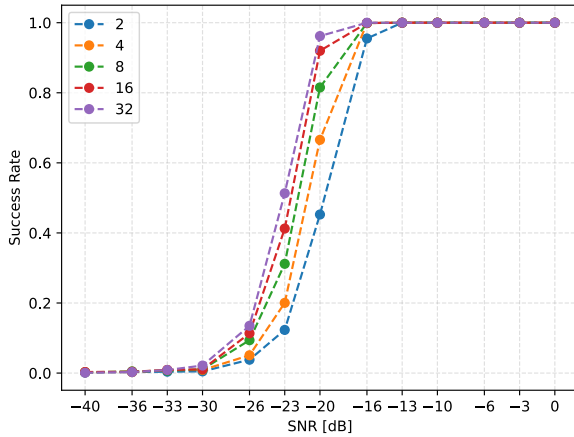
Fig. 7. Code acquisition success rate with decreasing signal-to-noise-ratio, for different integration times T given as multiples of the code length.
