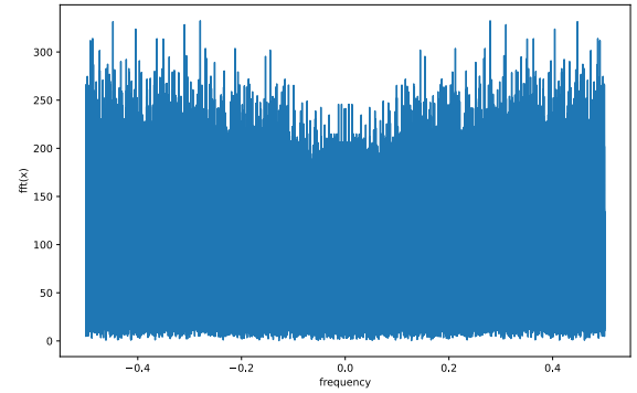
Fig. 8. Fourier transform of 1 \times 10^5 generated noise samples using the first configuration of LFSRs
