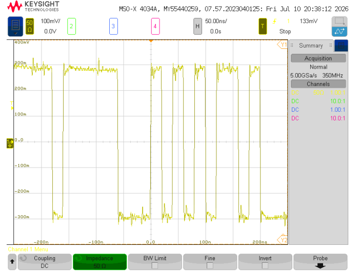
Fig. 11. Oscilloscope capture of the transmitter output signal.
