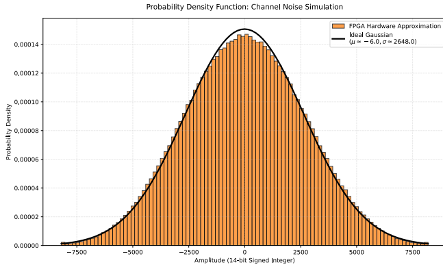
Fig. 10. Approximated PDF of generated noise. The extreme bins, containing the maximum and minimum of the 14-bit signed integer value, respectively, show a slightly inflated occurrence due to the applied saturating addition function.
