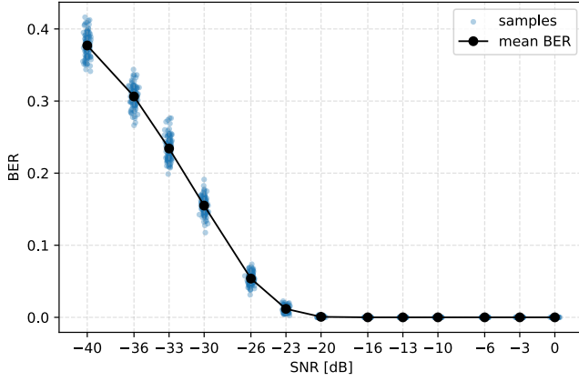
Fig. 6. BER of ideal receiver with decreasing signal-to-noise-ratio, assuming successful code acquisition.
