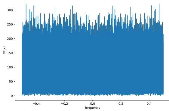
Fig. 9. Fourier transform of 1 \times 10^5 generated noise samples using the optimized configuration.
