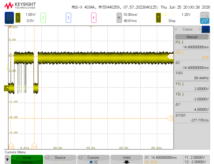
Fig. 16. Capture of the receiver data output during initial code acquisition. The transmitted data bit is fixed to “1”. During code acquisition, the receiver attempts to decode data from every candidate code offset as they are found, so random data is output until finally the correct code offset is acquired and locked onto.
