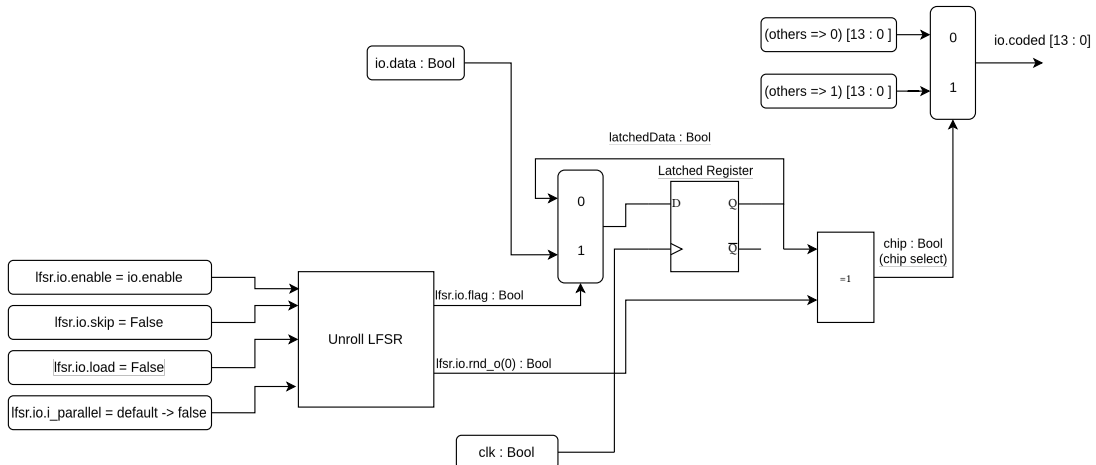
Fig. 2. Transmitter block diagram
