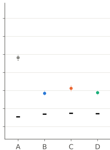
GPT-OSS-120B
