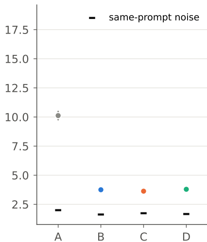
Claude Haiku 4.5
