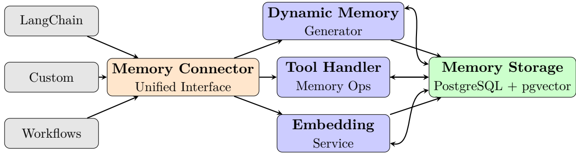
Figure 3: OAK.memory system architecture showing the connector pattern enabling framework-agnostic integration with diverse AI systems.
