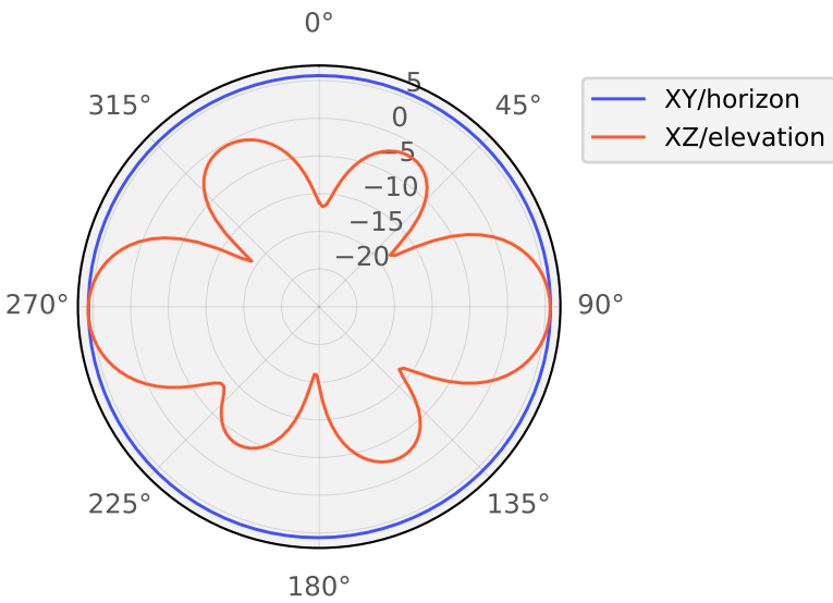
XY and XZ realized gain at 869.5 MHz (dBi)
