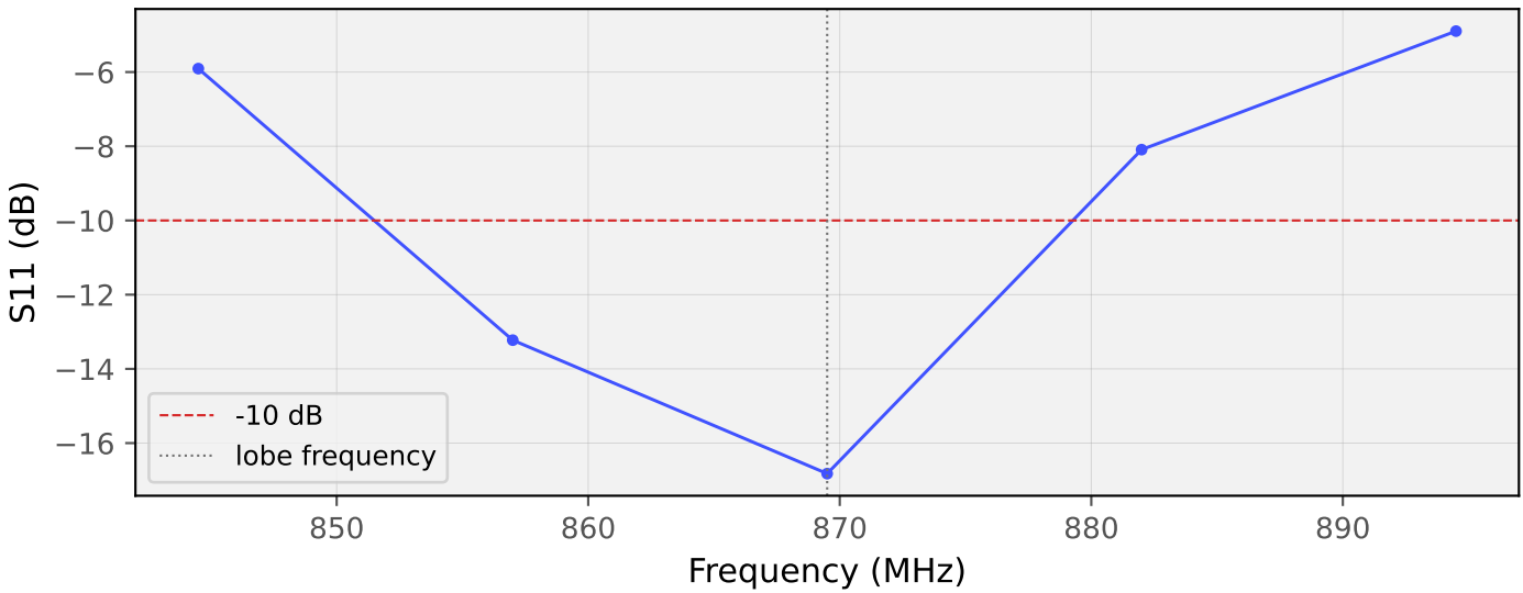
S11 sweep
