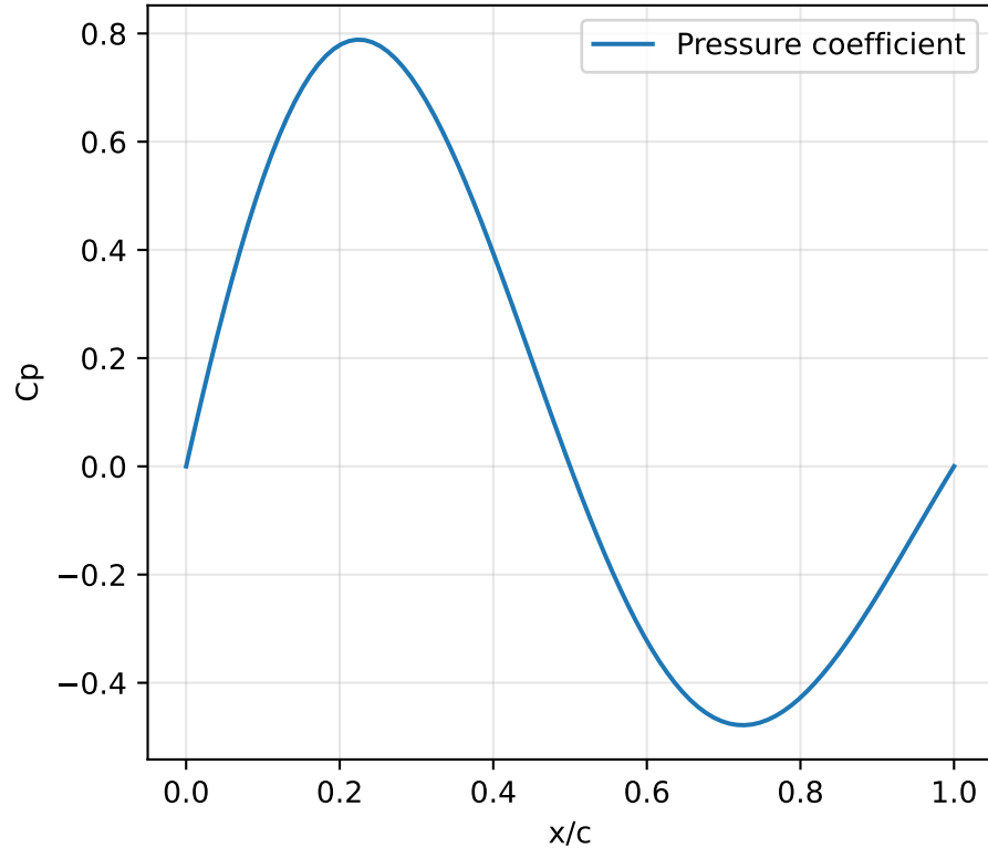
Pressure Distribution
