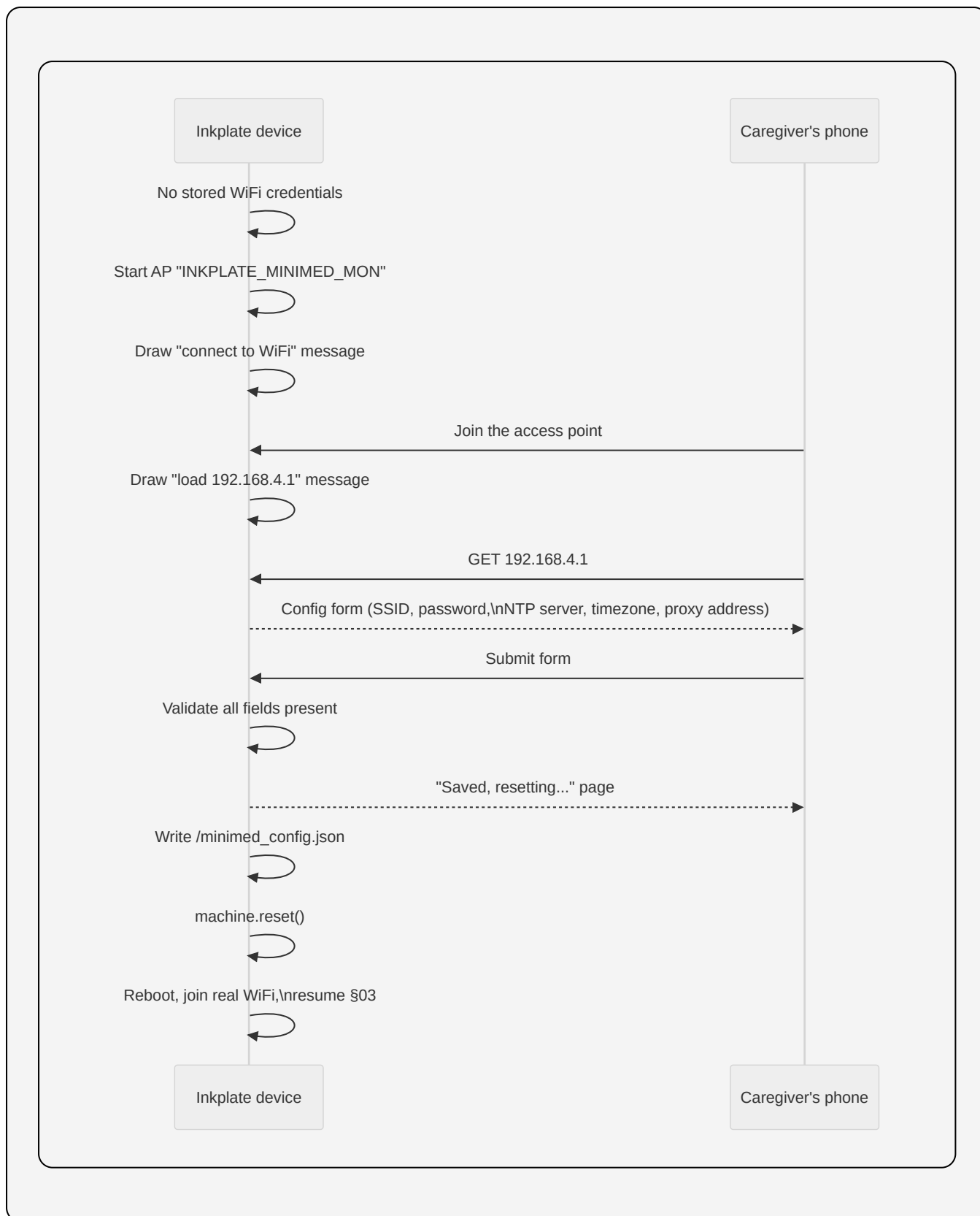
FIGURE 3 · ACCESS-POINT SETUP
