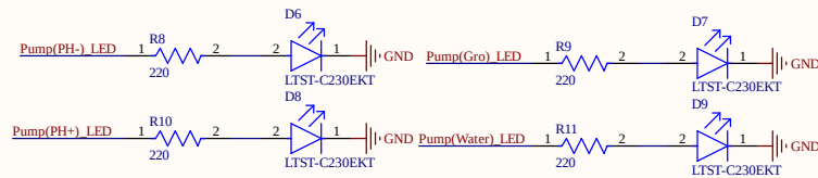
PUMP WARNING LIGHTS
