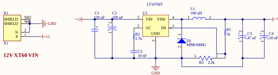
12-7V CONVERTOR
