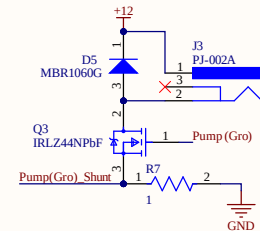
PUMP CONNECTORS
