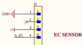
EC Sensor Connector
