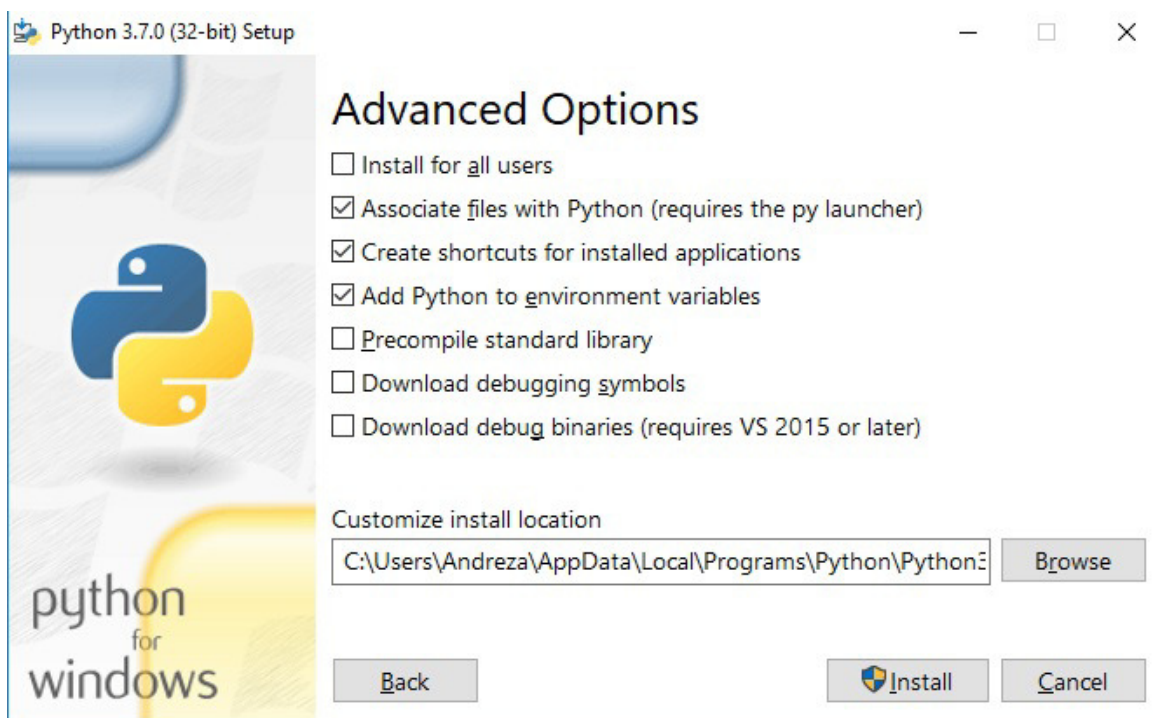
Figura 16.5: Advanced Options
