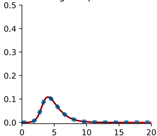
negative binomial network, high dispersion
