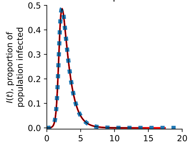
Poisson network, no dispersion
