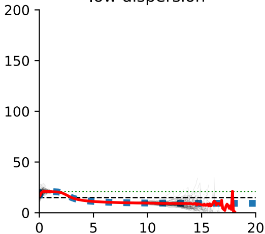
negative binomial network, low dispersion
