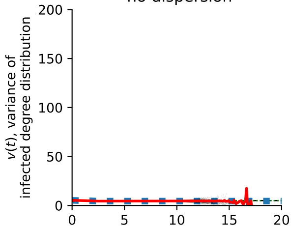
Poisson network, no dispersion
