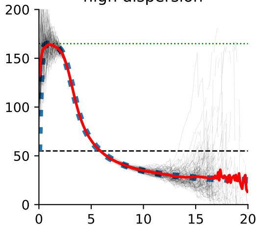
negative binomial network, high dispersion
