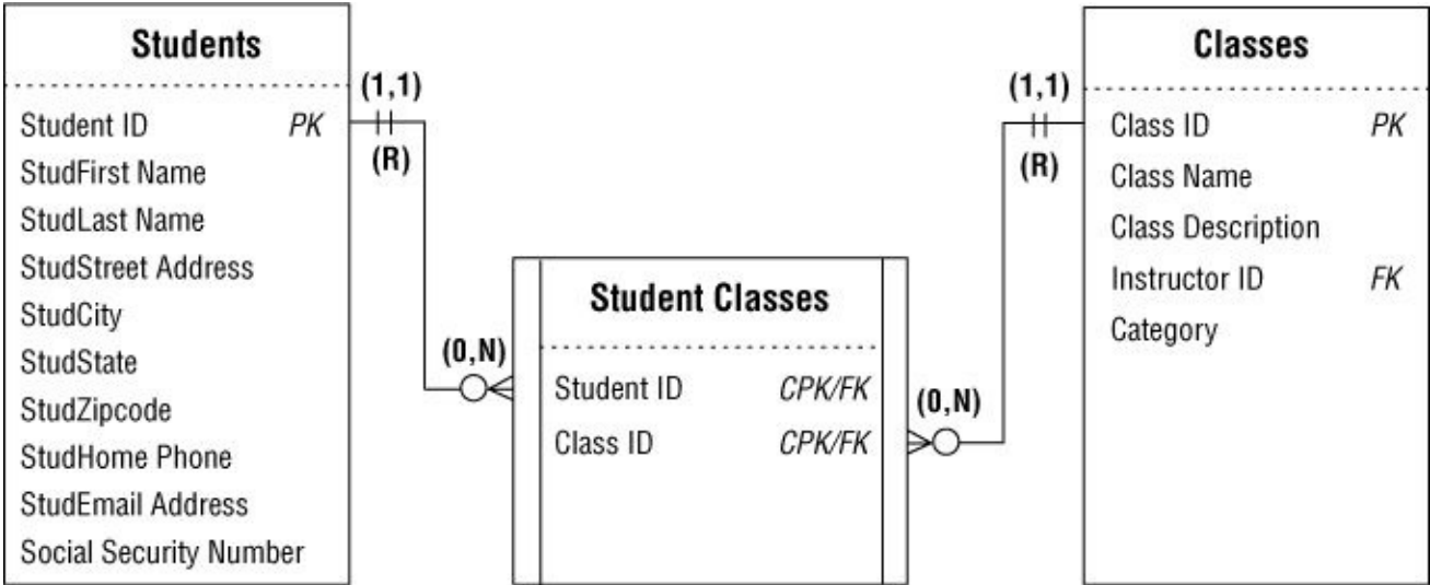
Figure 11.4. Tables and relationships from a school database
