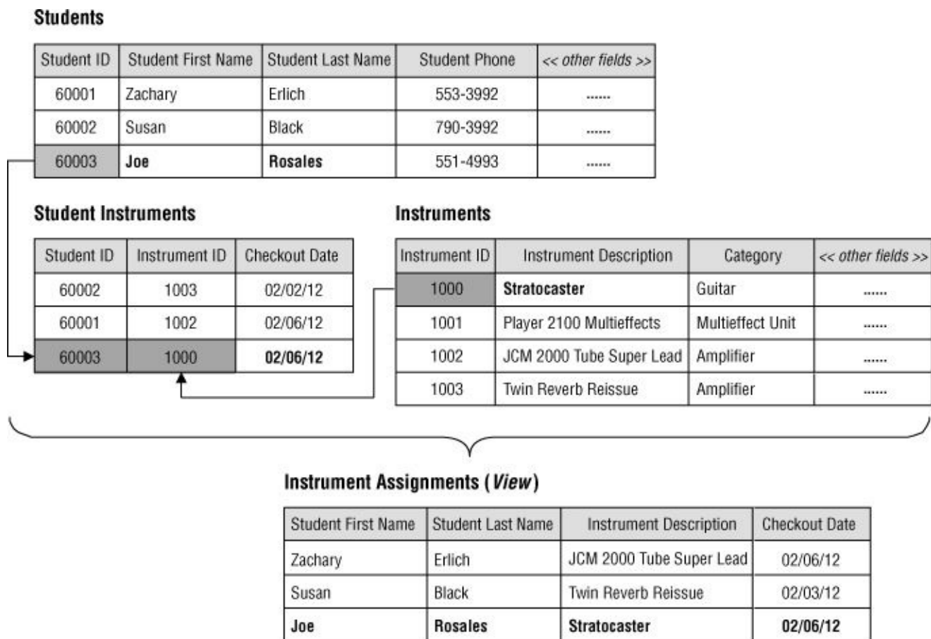
Figure 3.10. An example of a typical view
