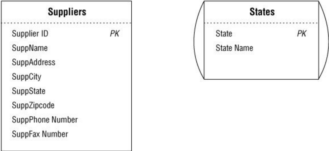
Figure 11.14. The SUPPLIERS table and the STATES validation table
