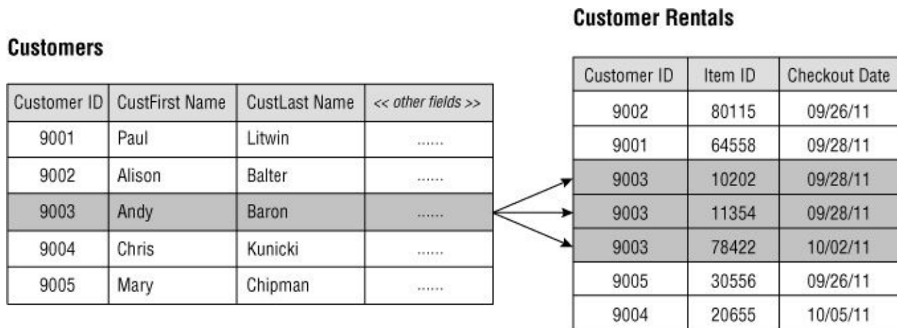
Figure 10.9. A typical example of a one-to-many relationship
