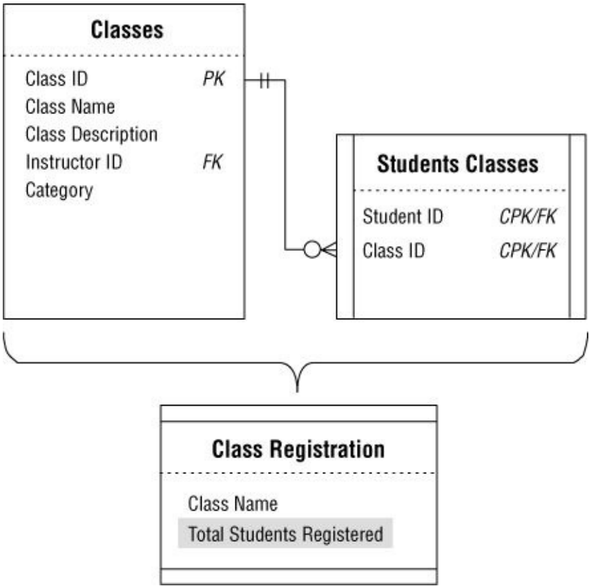
Figure 12.8. Revised diagram for the CLASS REGISTRATION view
