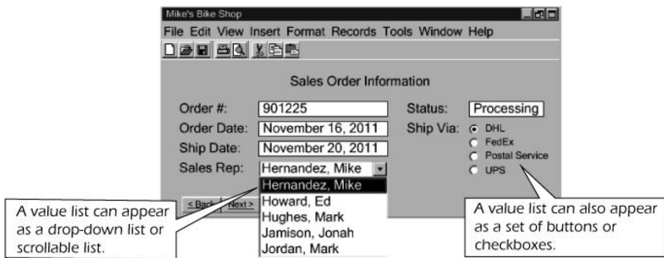
Figure 6.16. A database screen with two value lists
