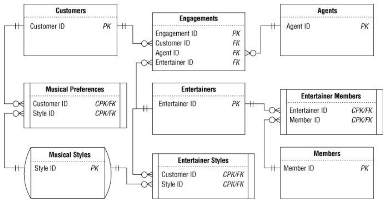
Entertainment Agency Database
