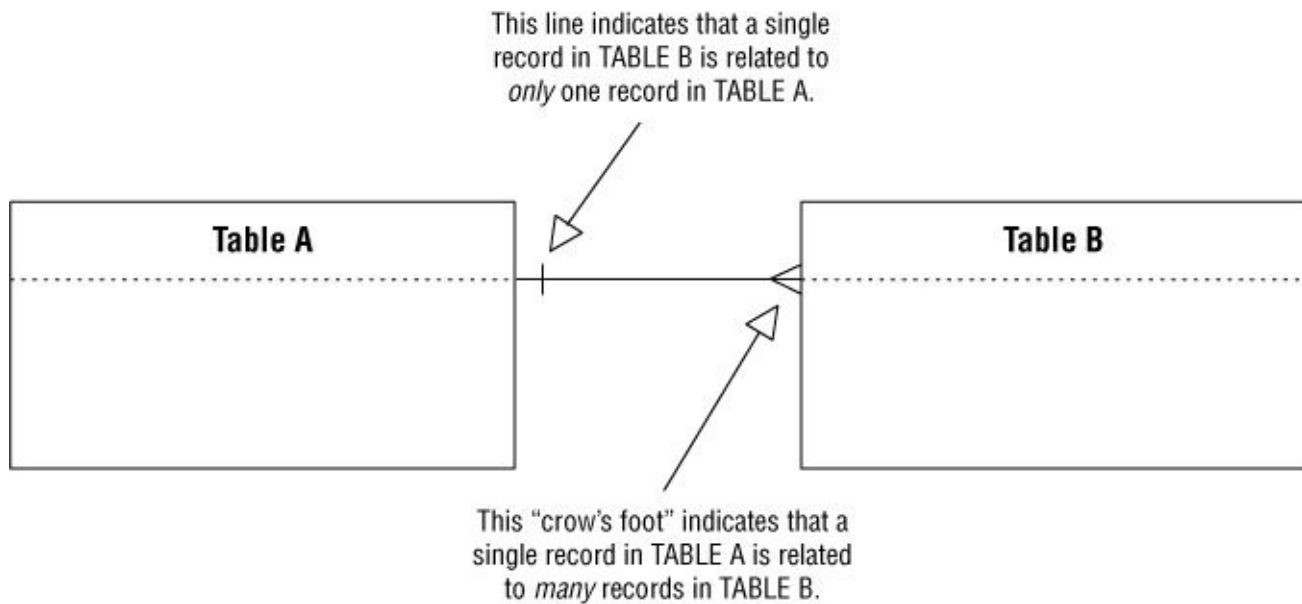
Figure 10.10. Diagramming a one-to-many relationship
