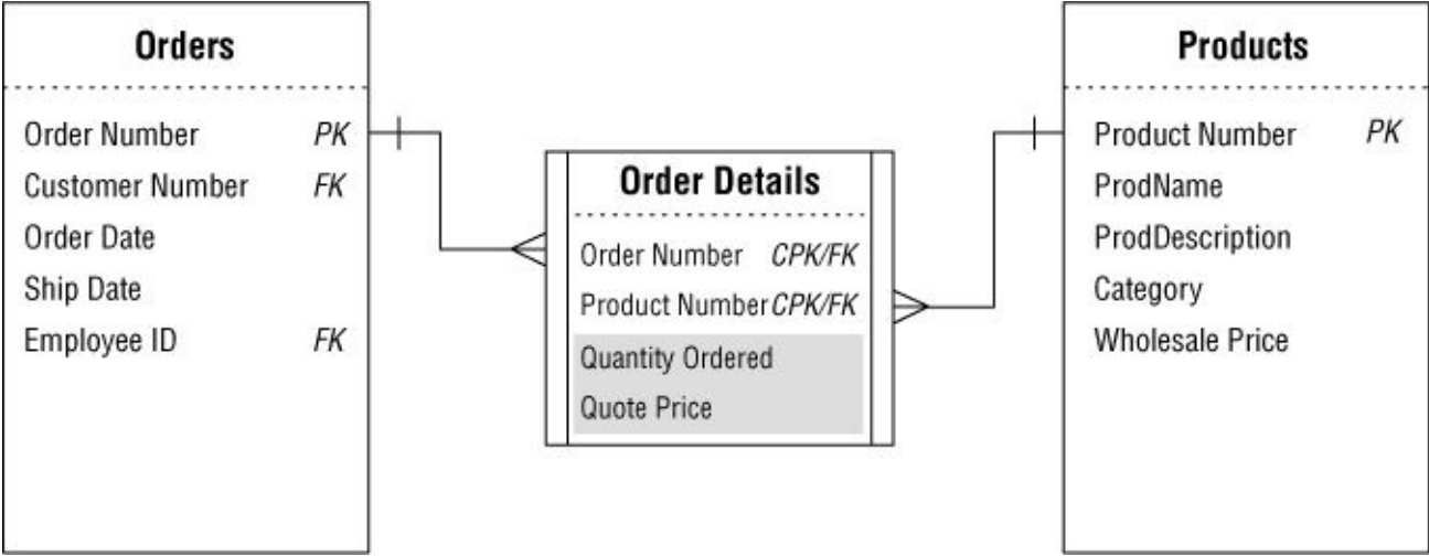
Figure 10.44. The revised ORDER DETAILS linking table
