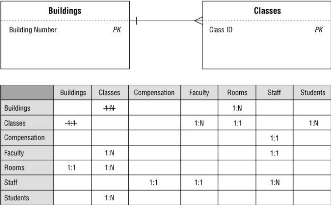
Figure 10.29. Identifying the official relationship between the BUILDINGS and CLASSES tables
