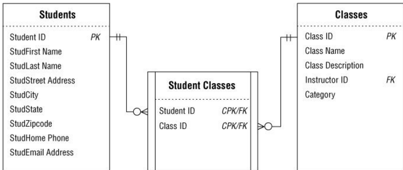
Figure 12.3. Base tables for the CLASS ROSTER view
