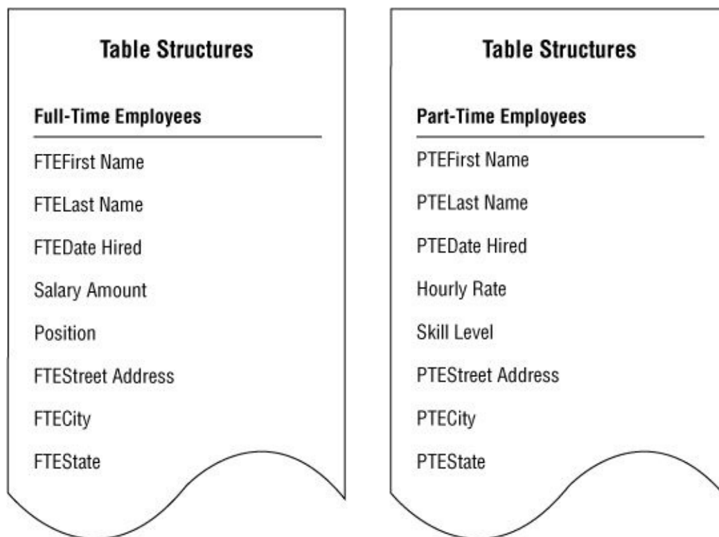
Figure 7.30. Previously unidentified subset tables
