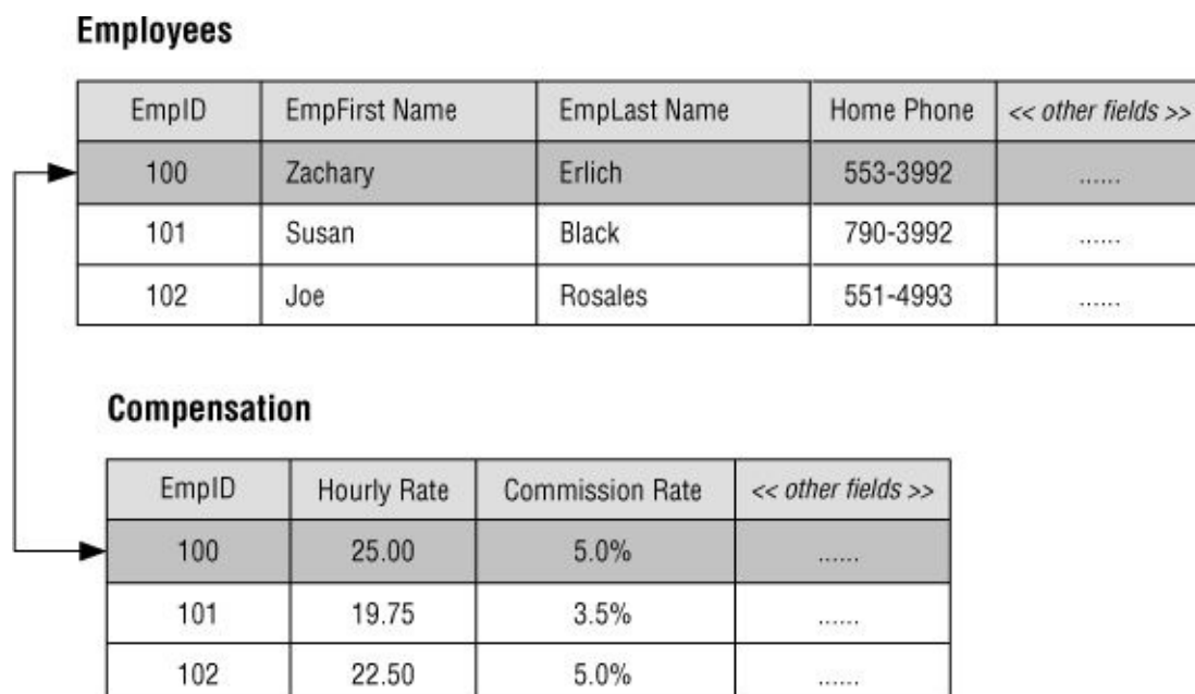
Figure 10.4. A typical example of a one-to-one relationship
