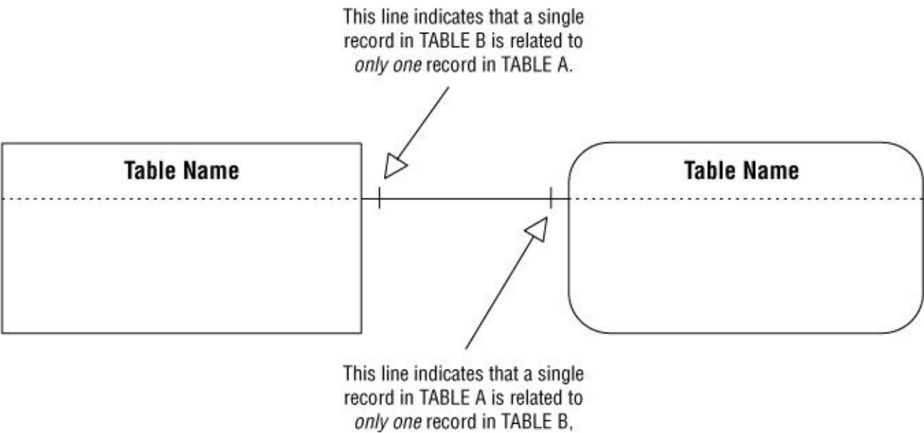
Figure 10.5. Diagramming a one-to-one relationship
