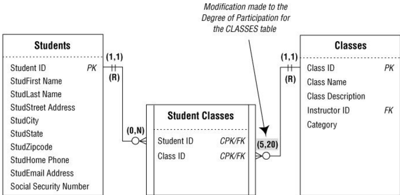
Figure 11.5. Establishing a relationship-specific business rule
