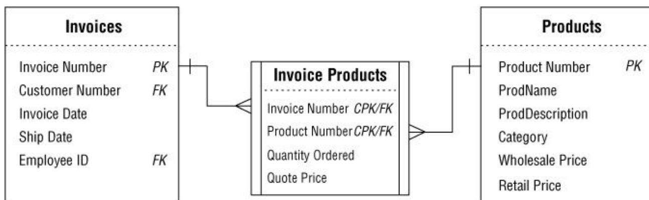
Figure 10.67. Establishing and diagramming the many-to-many relationship between the INVOICES and PRODUCTS tables
