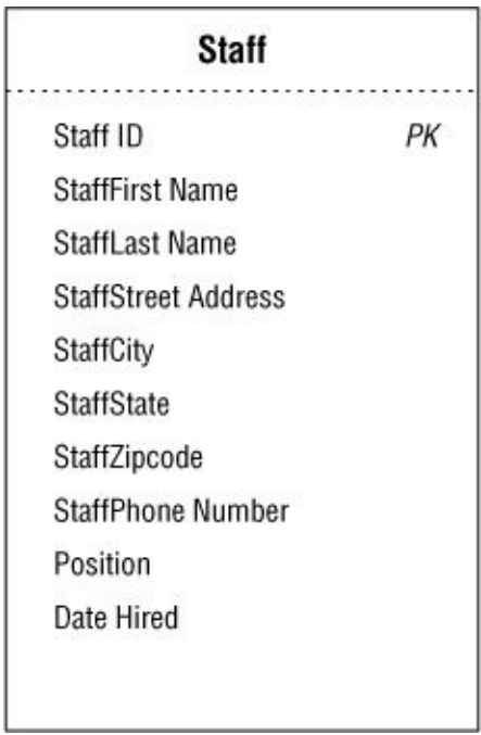
Figure 10.46. The current structure of the STAFF table
