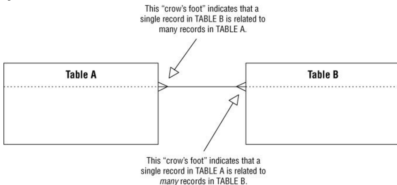
Figure 10.14. Diagramming a many-to-many relationship
