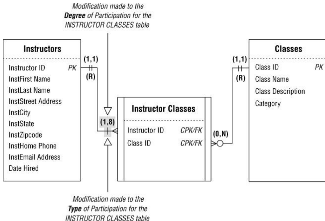
Figure 11.10. The revised relationship diagram that establishes the new business rule
