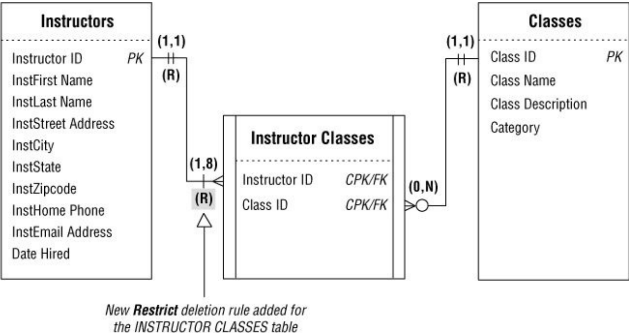
Figure 11.11. Establishing a Restrict deletion rule for the INSTRUCTOR CLASSES table to support the new business rule
