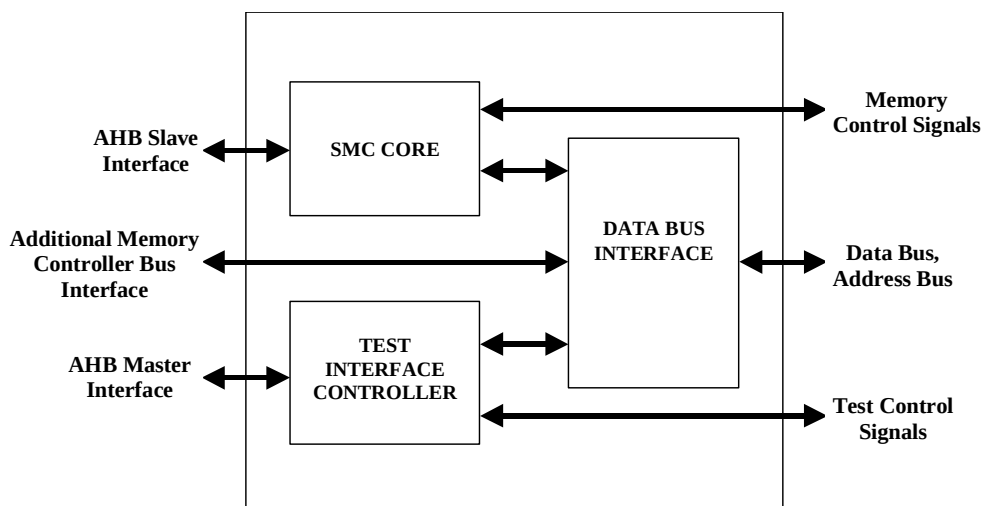
Figure 5-1: ARM PrimeCell Static Memory Controller block diagram
