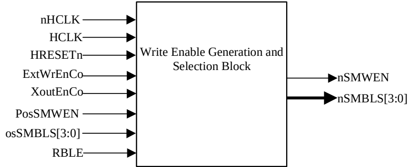
Figure 6.3-3 Write Enable Generation and Selection Block
