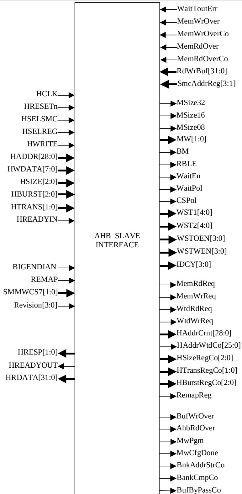
Figure 6.1-1 AHB Interface block
