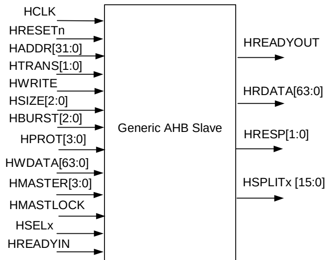
Figure 10.1-1 Generic AHB Slave Block diagram
