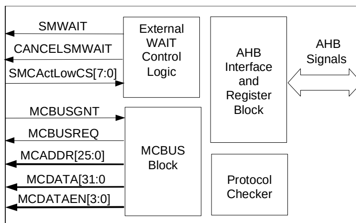
Figure 9.1-1 SMC Trickbox Block Diagram
