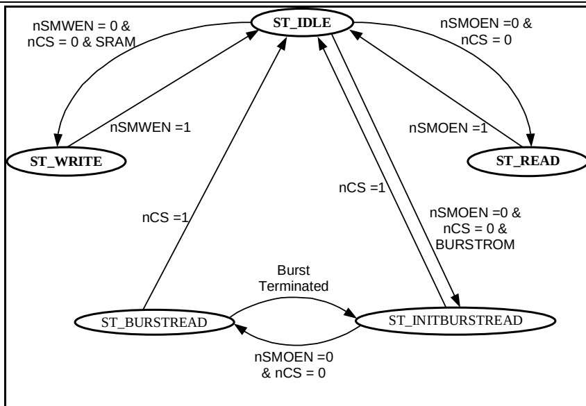
Figure 9.2-2 TrickMem state machine
