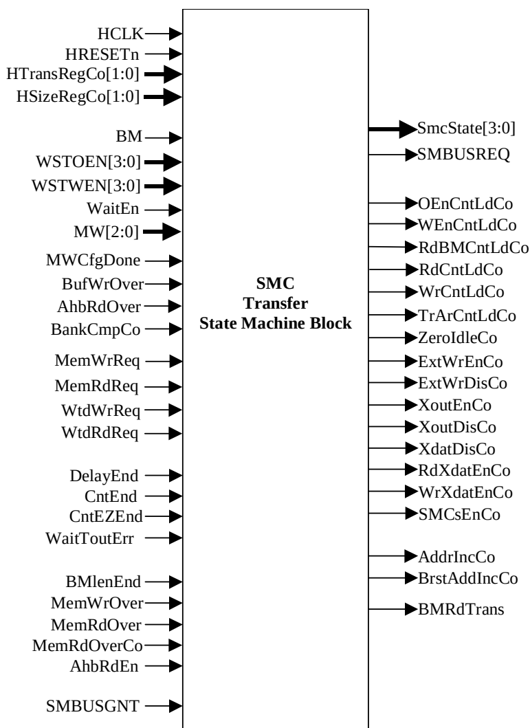
Figure 6.2-2 Transfer State Machine block
