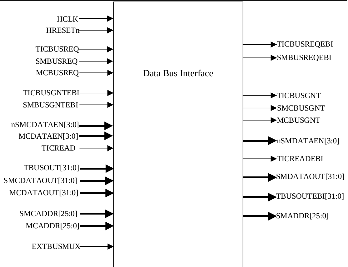
Figure 7.2-1 The Data Bus Interface [DBI] Block
