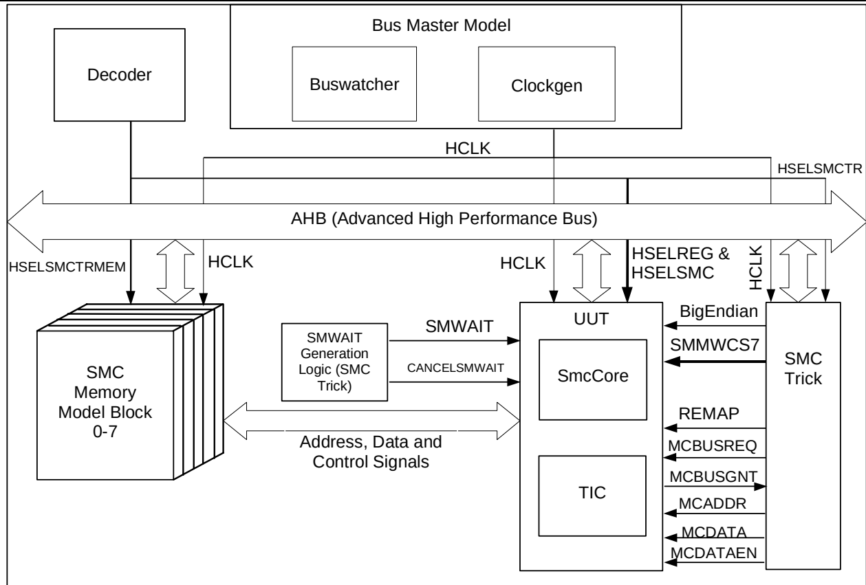
Figure 8-1 SMC Functional Verification Testbench
