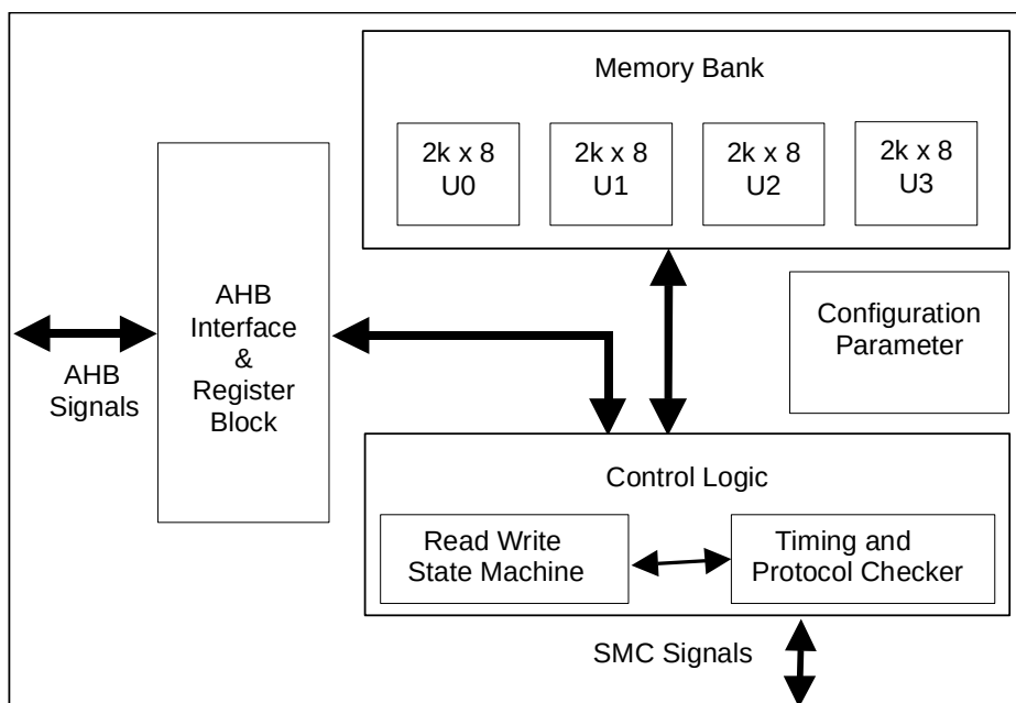
Figure 9.2-1 TrickMem block diagram
