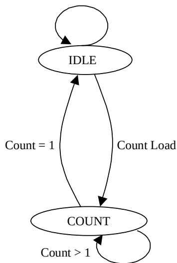
Figure 6.2.4 : DelayEnd generation state diagram
