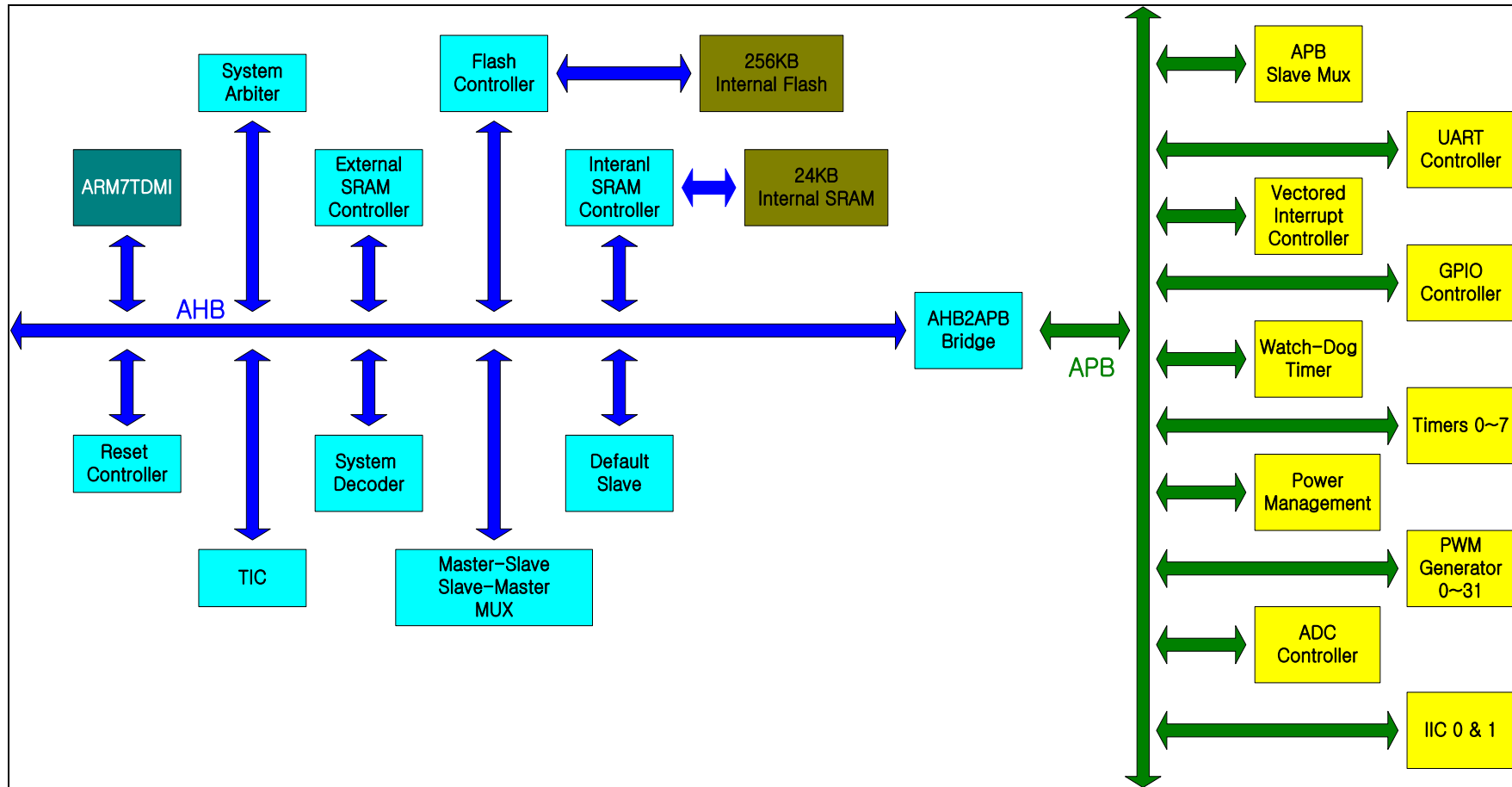
Fig. DTSDI003 Block diagram
