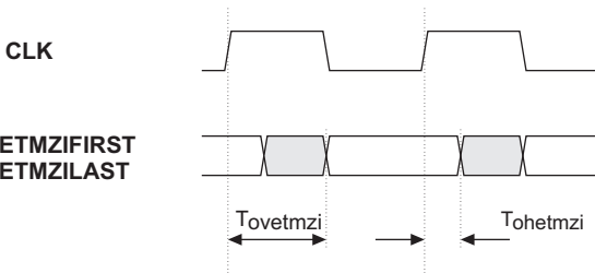
Figure 9-10 ETMZIFIRST and ETMZLAST interface timing
