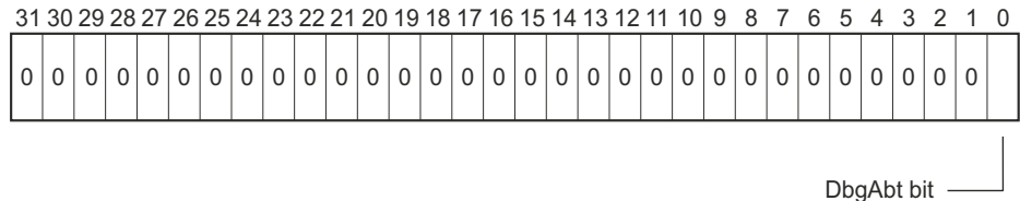
Figure 6-9 Coprocessor 14 monitor mode debug status register format
