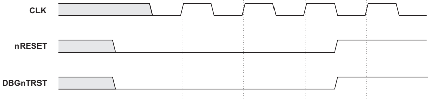
Figure 7-1 System reset
