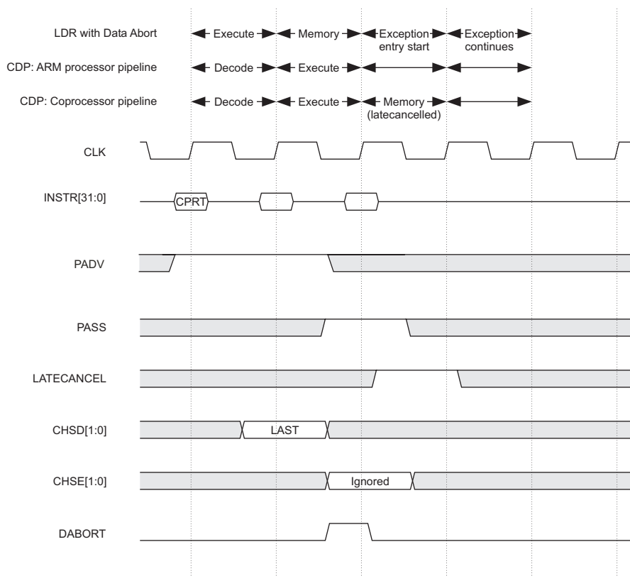
Figure 5-7 ARM9EJ-S core late-cancelled CDP
