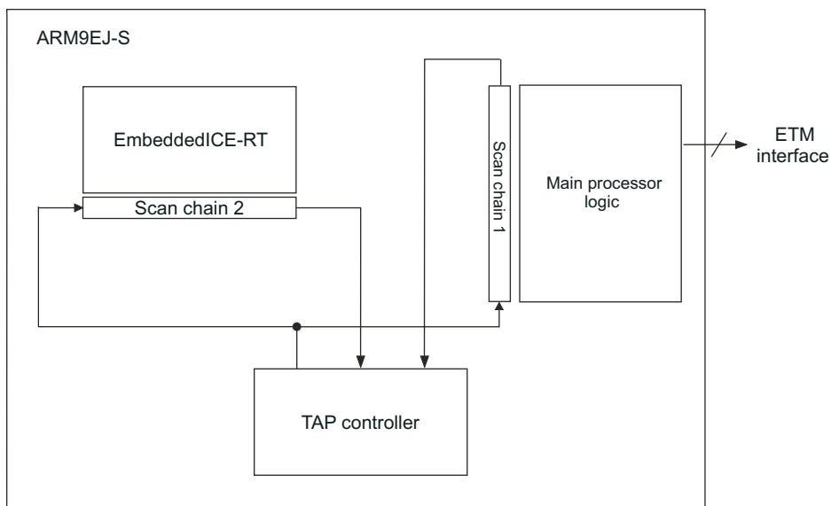
Figure B-1 ARM9EJ-S core scan chain arrangements
