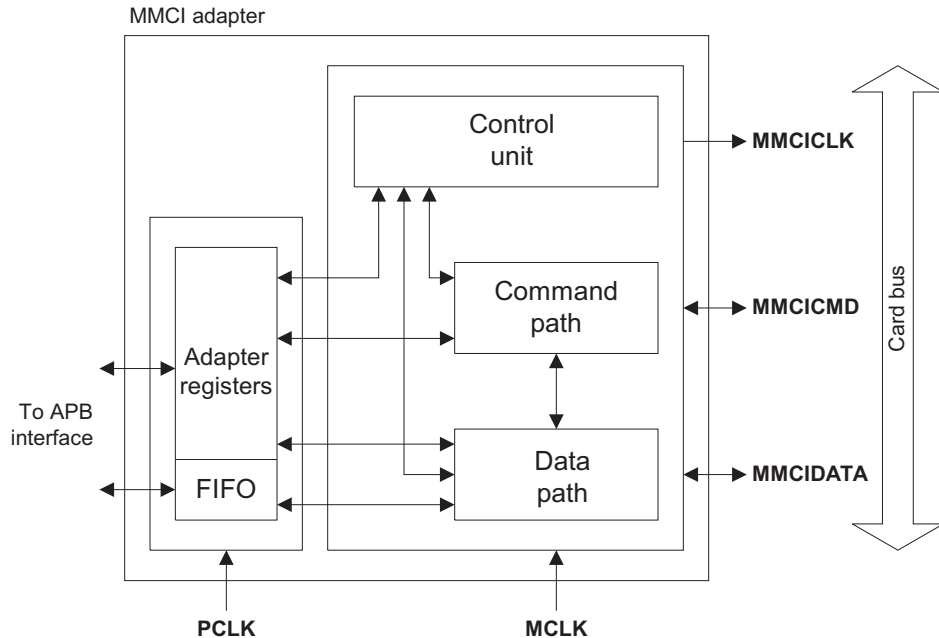
Figure 2-2 PrimeCell MMCI Adapter
