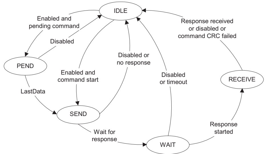
Figure 2-5 Command path state machine
