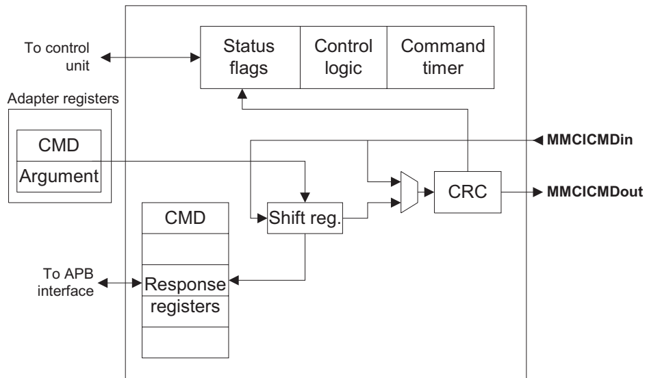
Figure 2-4 Command path
