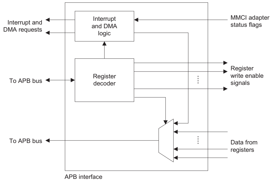
Figure 2-11 APB interface
