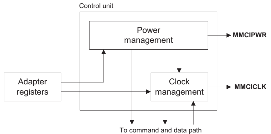
Figure 2-3 Control unit
