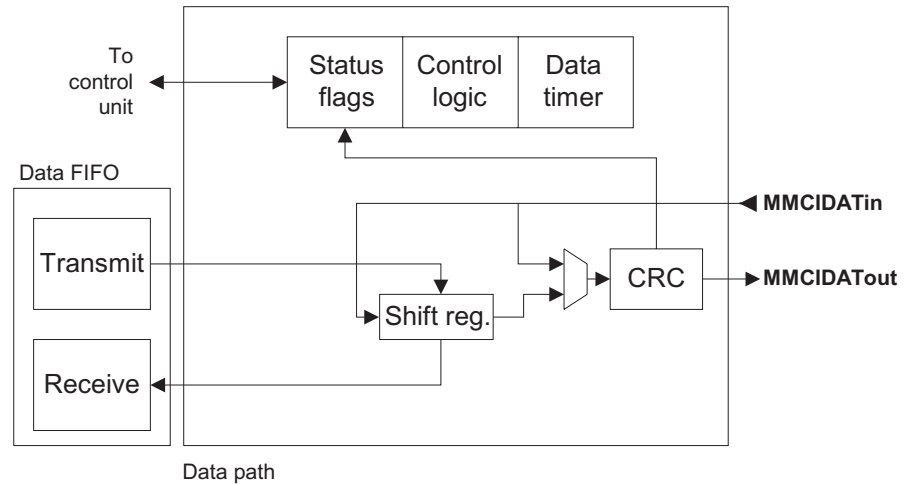
Figure 2-7 Data path
