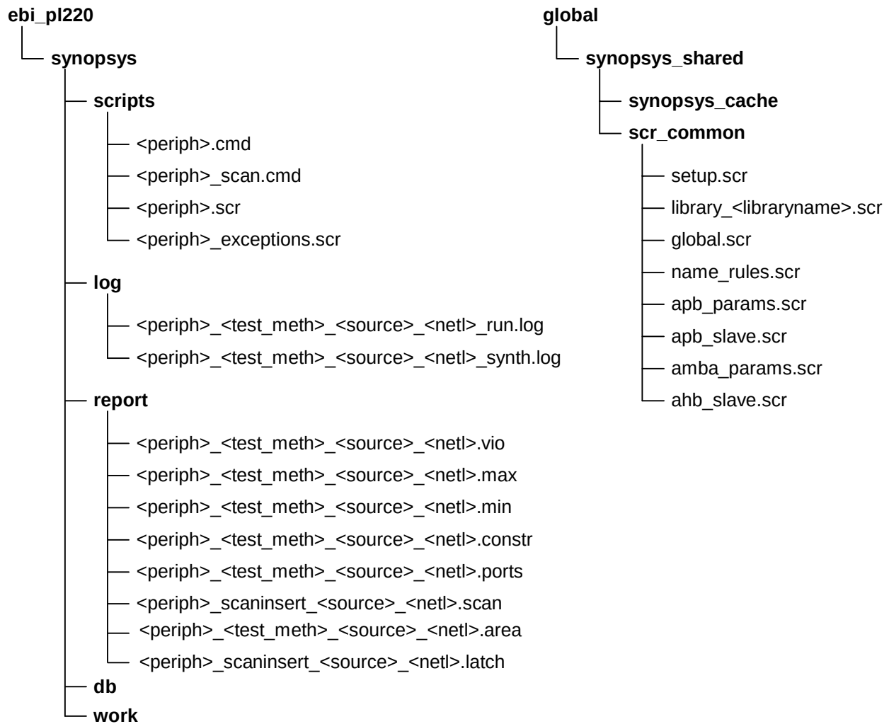
Figure 3-4. Generic Synopsys synthesis reference directory structure
