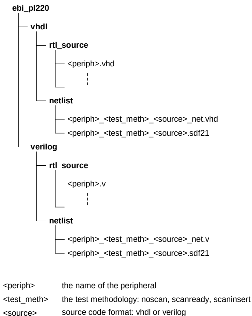
Figure 3-3. Source Code Directory Structure
