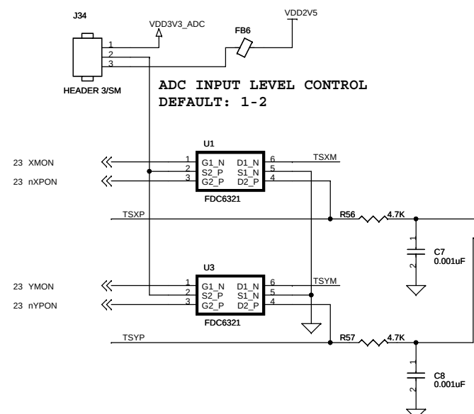
EXTERNAL ADC INPUT AND JUMPER
