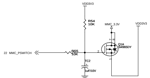
SD/HS-MMC SOCKET
