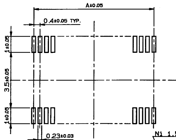
MOUNTING LAYOUT
