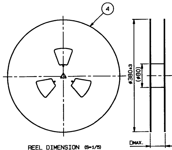
REEL DIMENSION (S-1/5)
