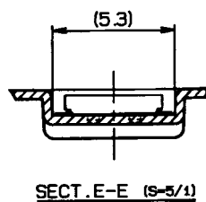
SECT. E-E (S-5/1)
