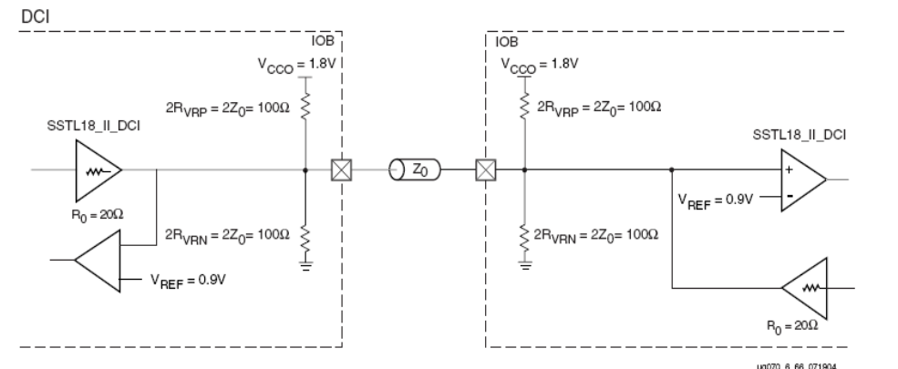
Figure 6-68: SSTL (1.8V) Class II Termination
