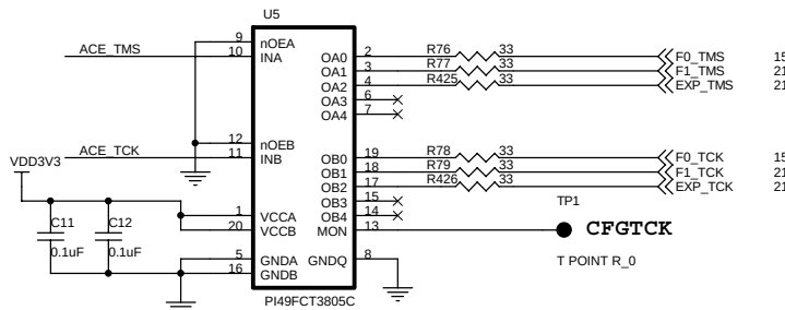
SYSTEMACE JTAG TCK/TMS BUFFER
