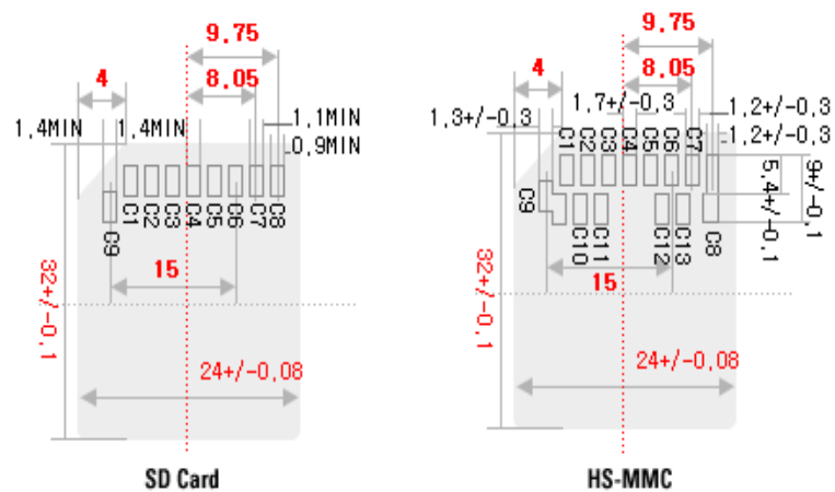
SD/HS-MMC SOCKET
