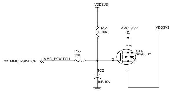
SD/HS-MMC SOCKET
