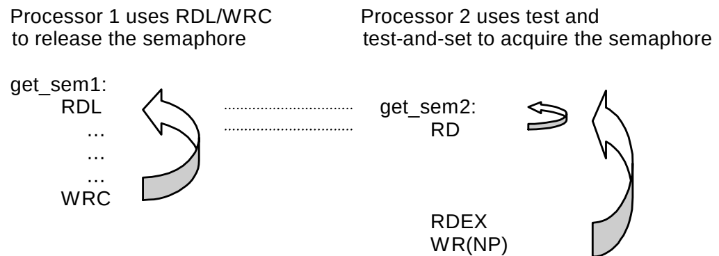
Figure 44 Correct Synchronization Sequence
