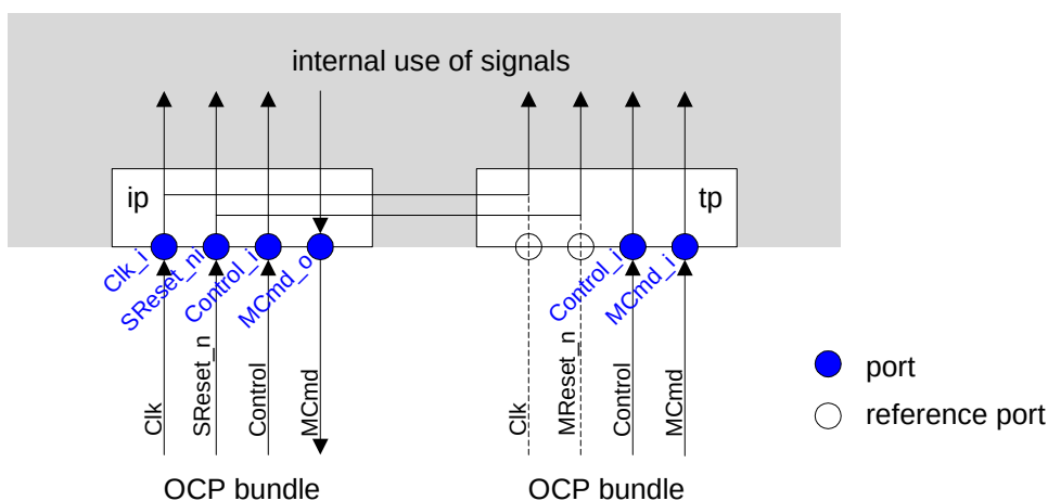
Figure 7 Reference Port
