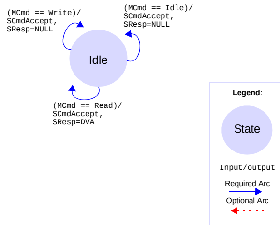
Figure 40 Combinational OCP Slave
