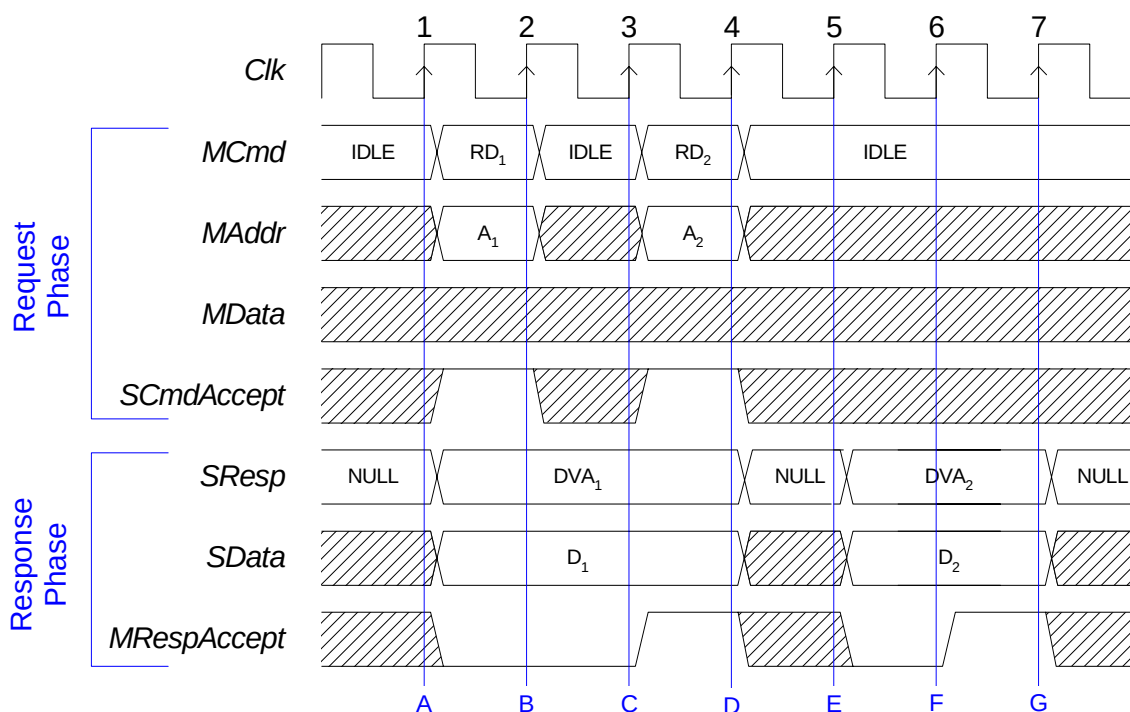
Figure 22 Response Accept
