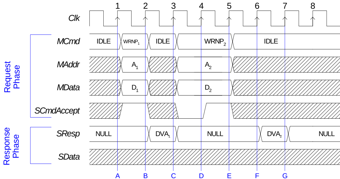
Figure 18 Non-posted Write
