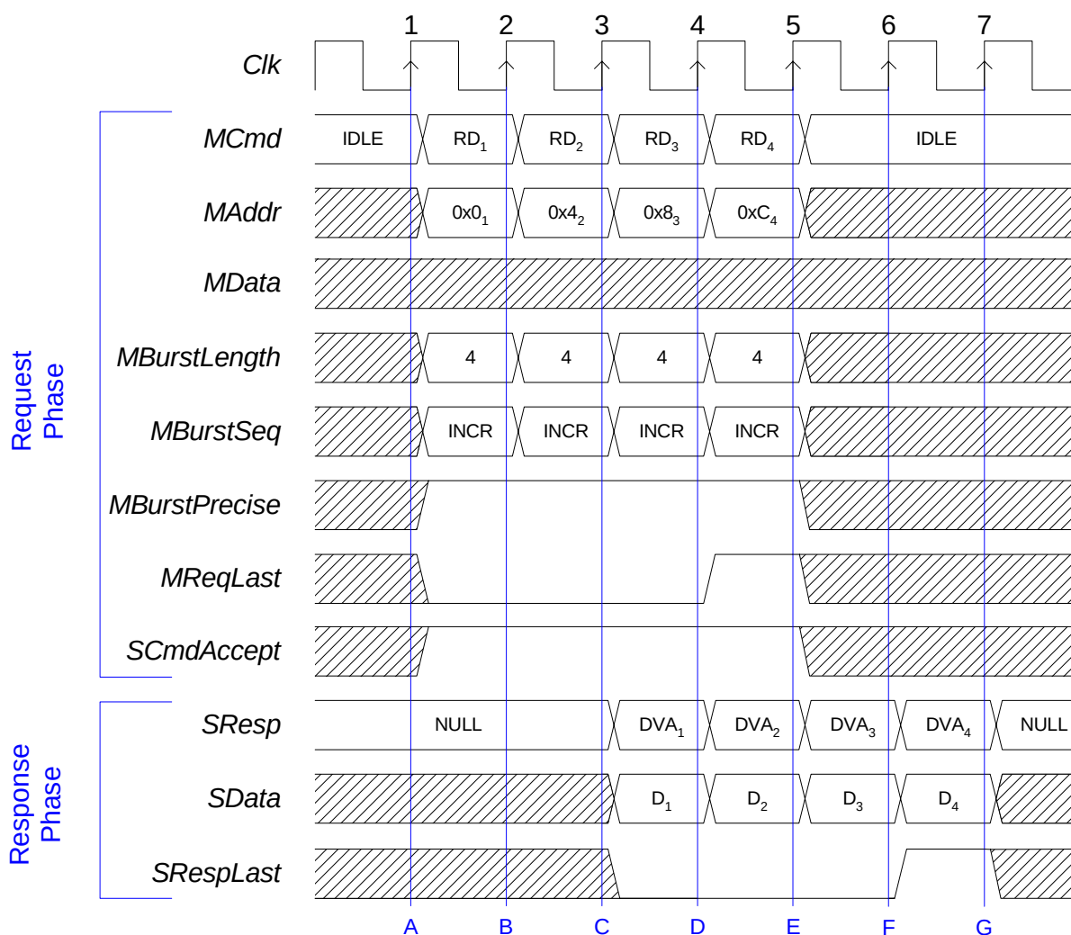
Figure 23 Incrementing Precise Burst Read
