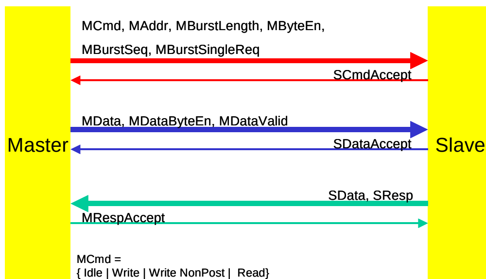
Figure 46 Block Data Flow Signal Processing
