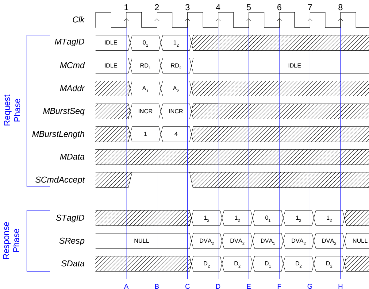
Figure 32 Tagged Burst Transactions
