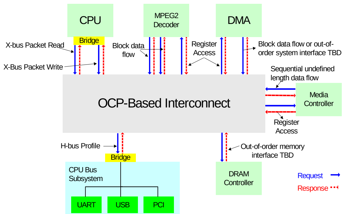
Figure 45 OCP Profiles
