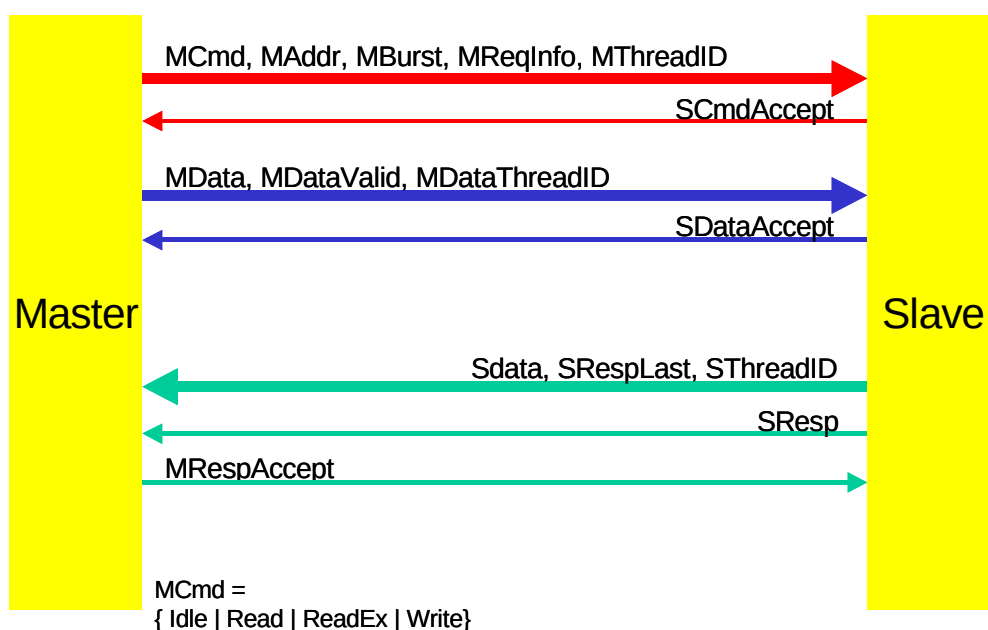
Figure 51 X-bus Packet Read Signal Processing
