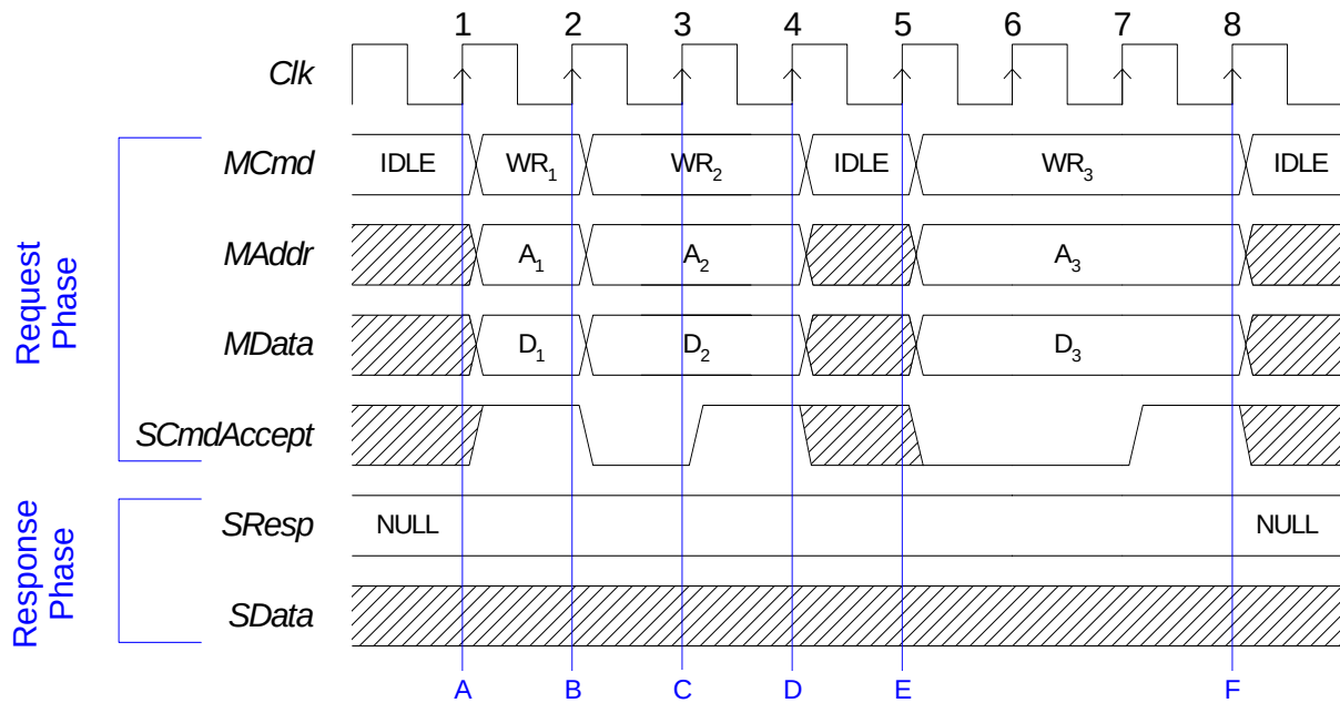
Figure 15 Request Handshake
