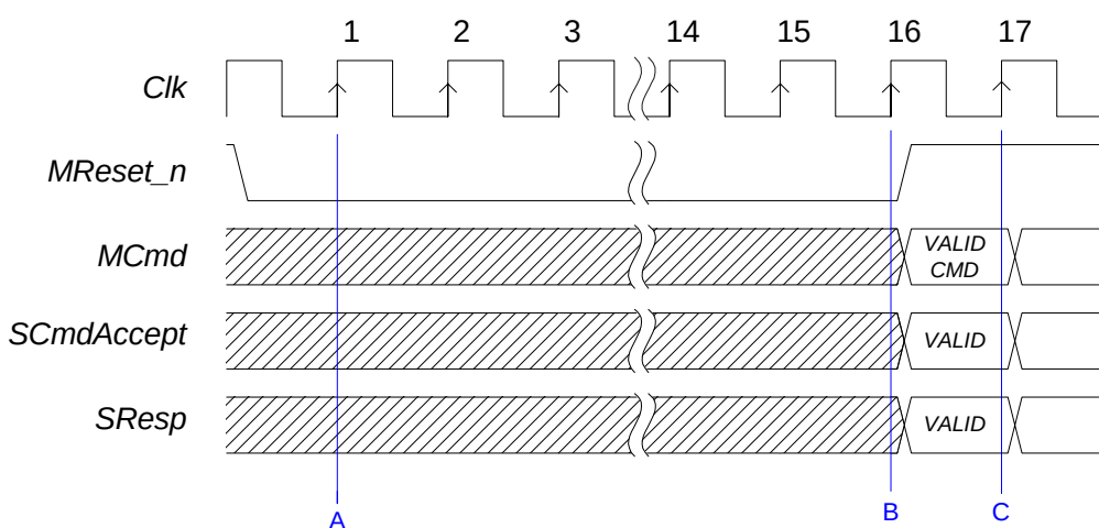
Figure 36 Reset Sequence
