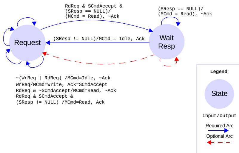
Figure 39 Combinational OCP Master
