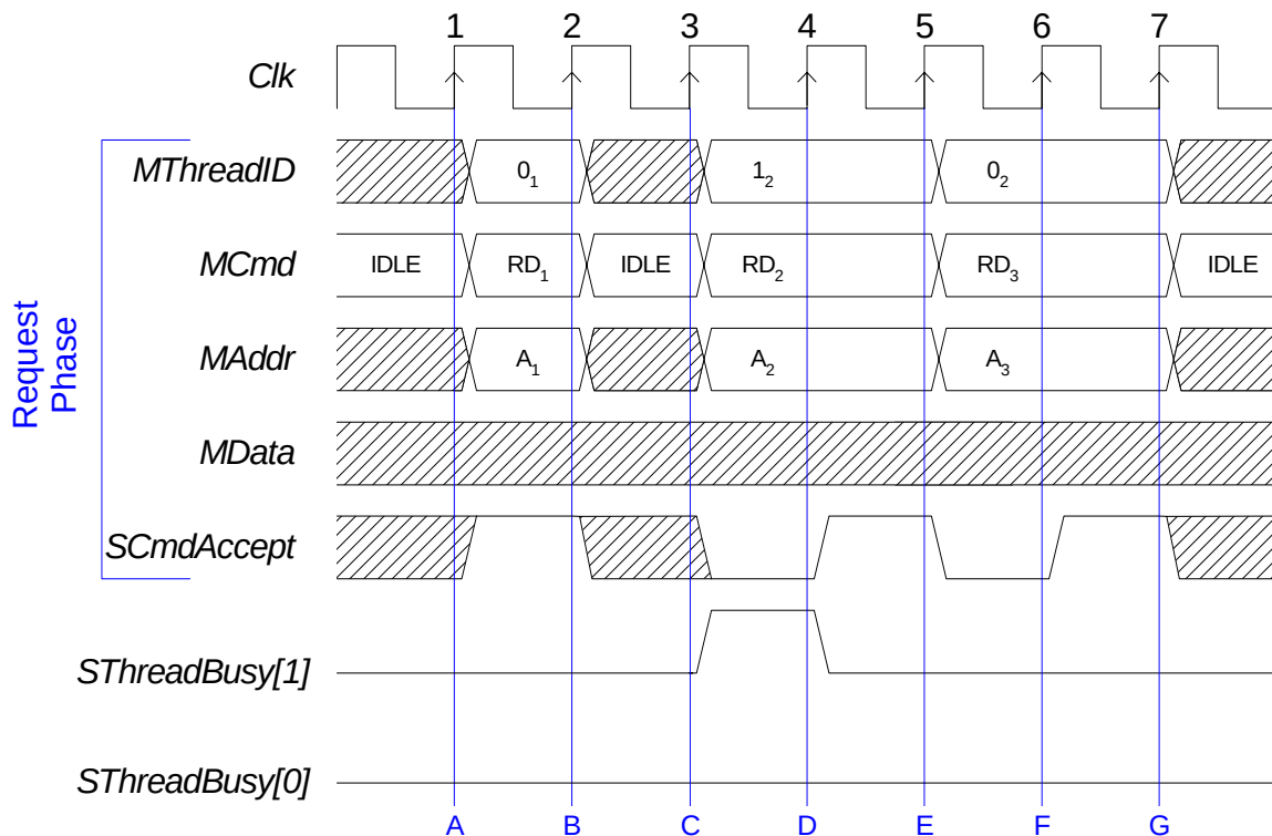
Figure 34 Threaded Read with Thread Busy
