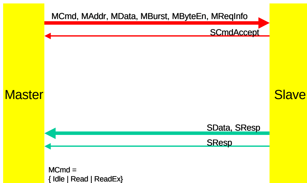
Figure 49 Simple H-Bus Signal Processing
