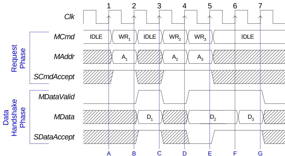
Figure 29 Datahandshake Extension
