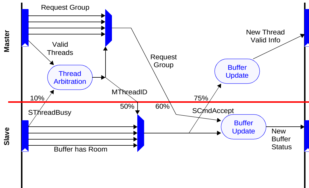
Figure 41 Multithreaded OCP Interface Implementation
