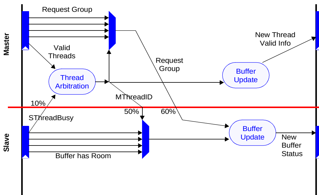
Figure 42 Multithreaded OCP Interface with threadbusy_exact
