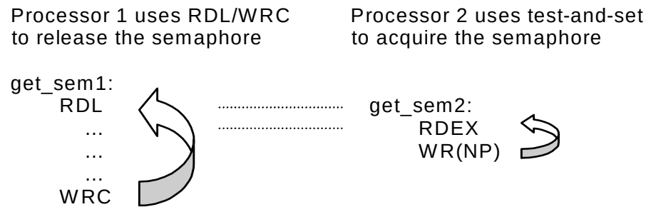
Figure 43 Synchronization Deadlock
