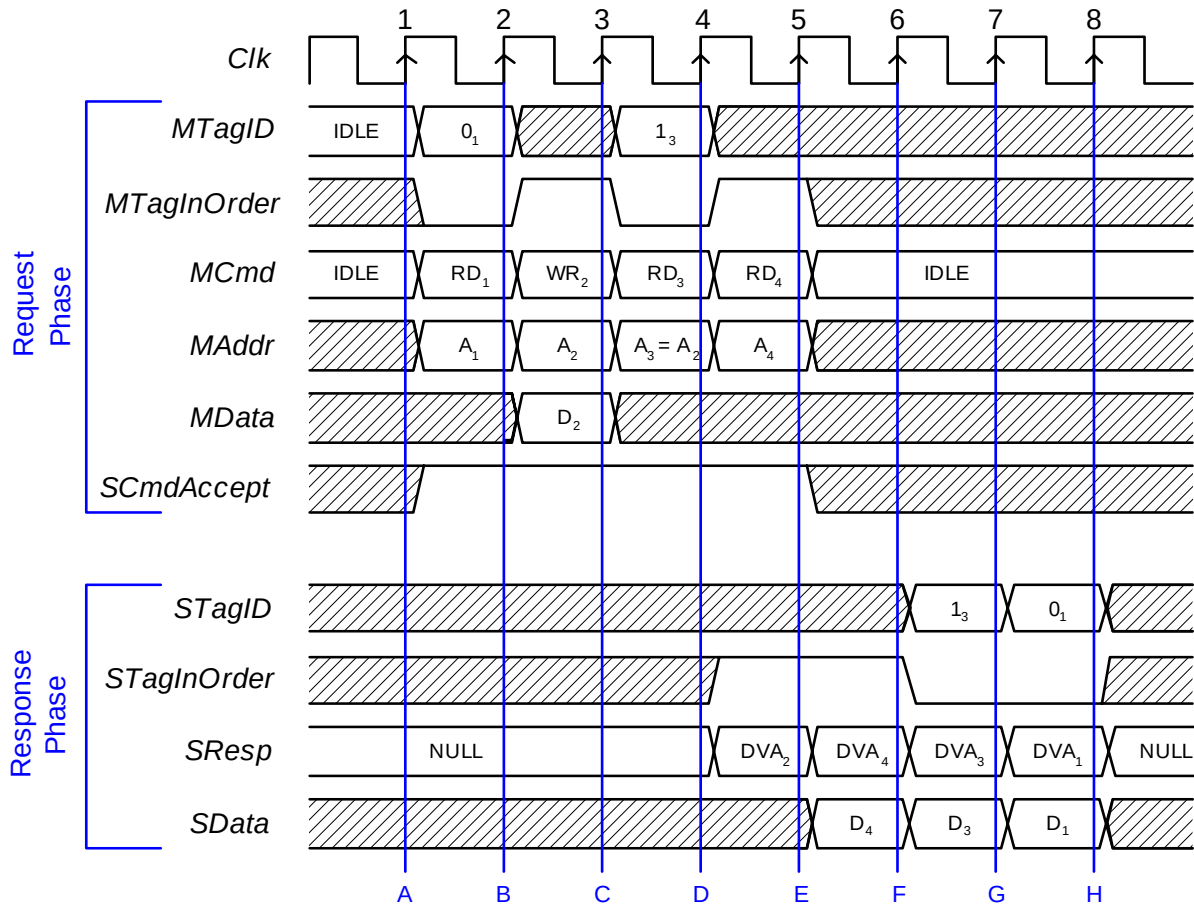
Figure 31 Tagged Reads
