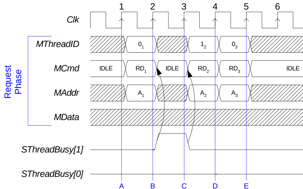
Figure 35 Threaded Read with Thread Busy Exact
