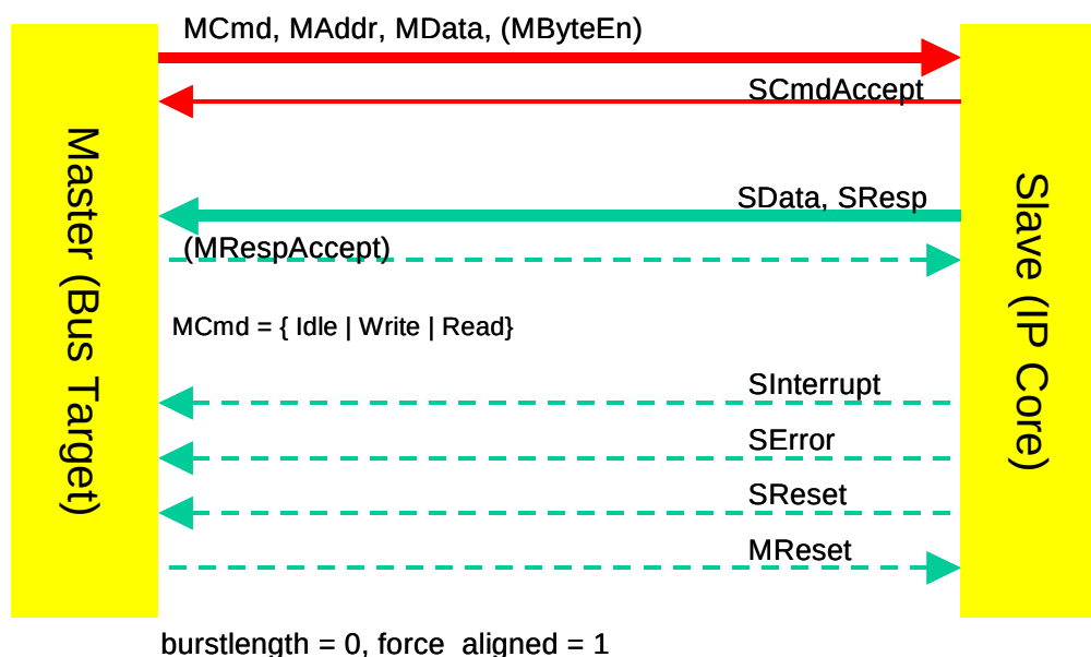
Figure 48 Register Access Signals Processing
