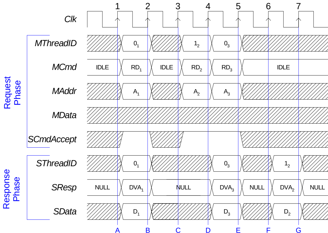
Figure 33 Threaded Read
