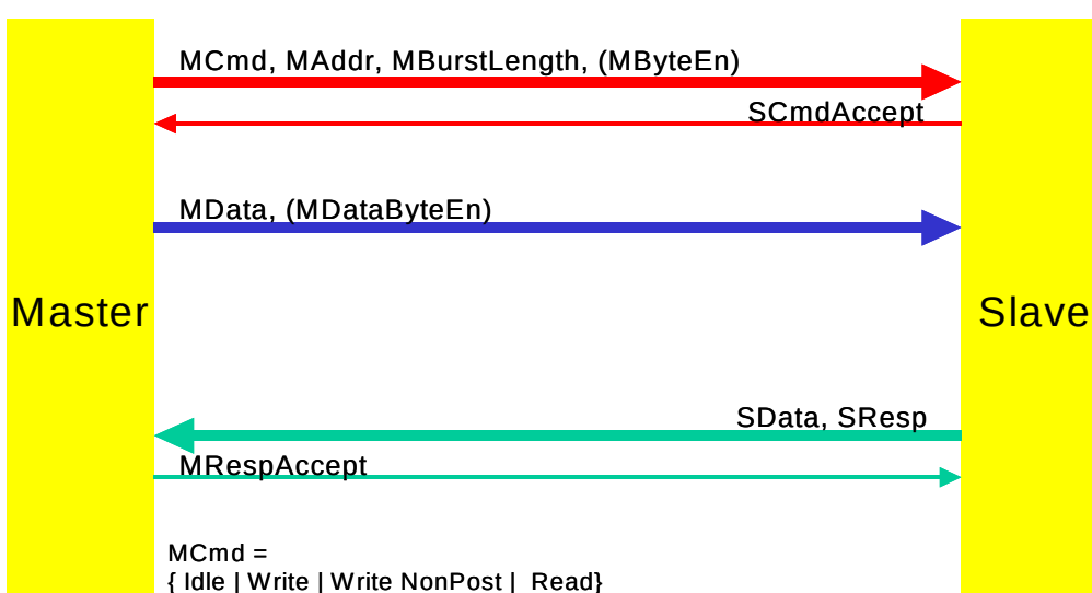
Figure 47 Sequential Undefined Length Data Flow Signals Processing
