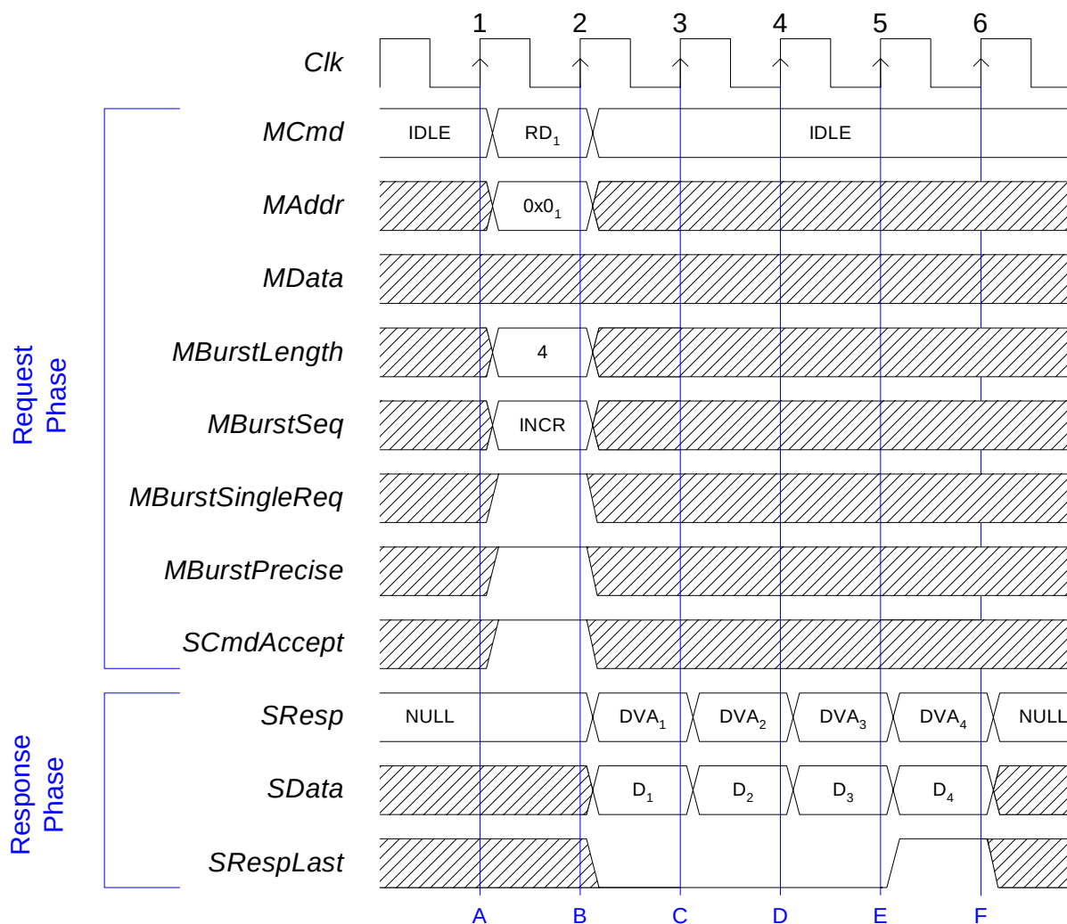
Figure 28 Single Request Burst Read
