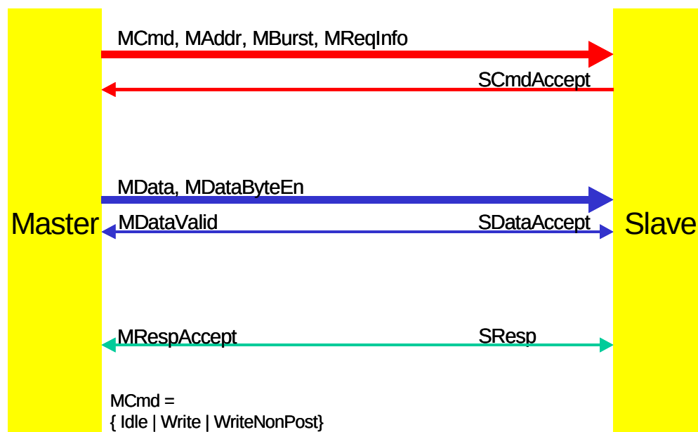
Figure 50 X-bus Packet Write Signal Processing
