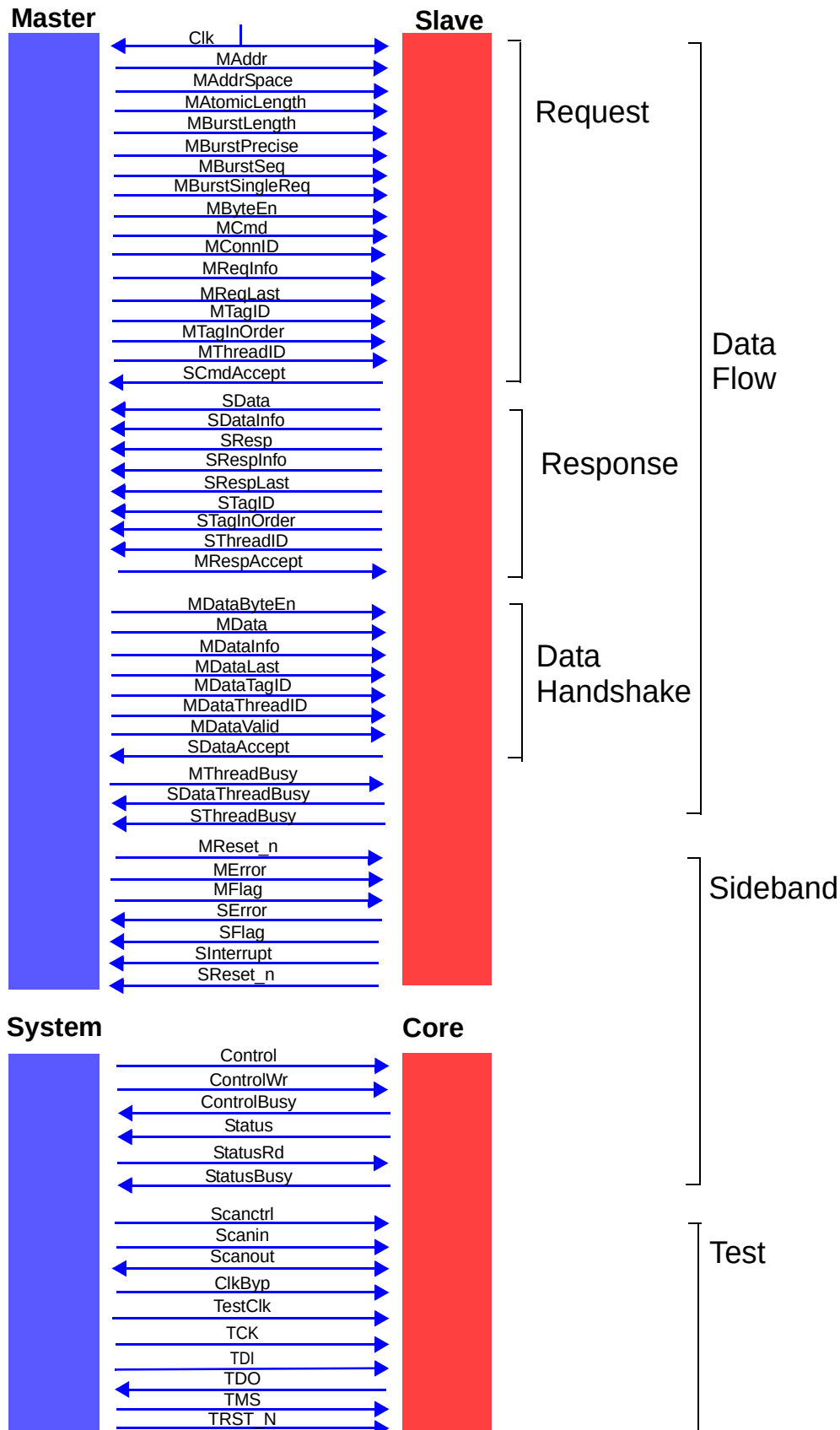
Figure 4 OCP Signal Summary
