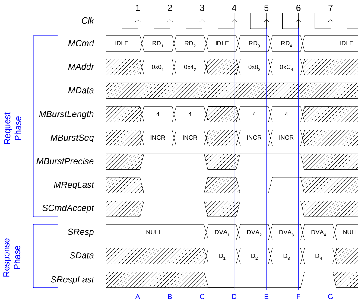
Figure 26 Incrementing Precise Burst Read with IDLE Cycle
