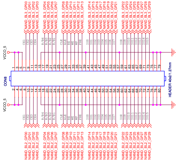
Test Header Pin
