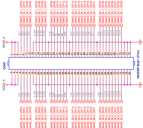
Nand Flash Board Connector
