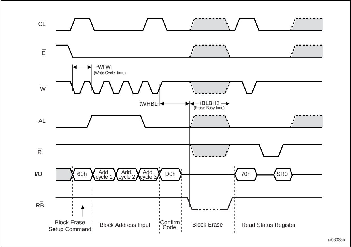
Figure 26. Block Erase AC waveform
