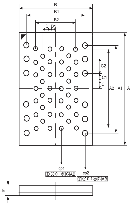
Figure 32. 52-ULGA, 12 x 17mm, Package Outline (Top view through package)
