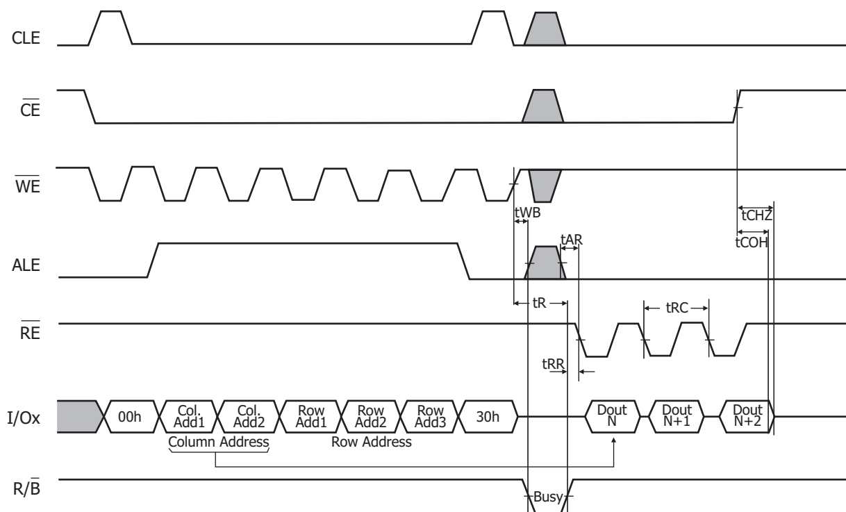
Figure 11: Read1 Operation intercepted by \overline{\text{CE}}
