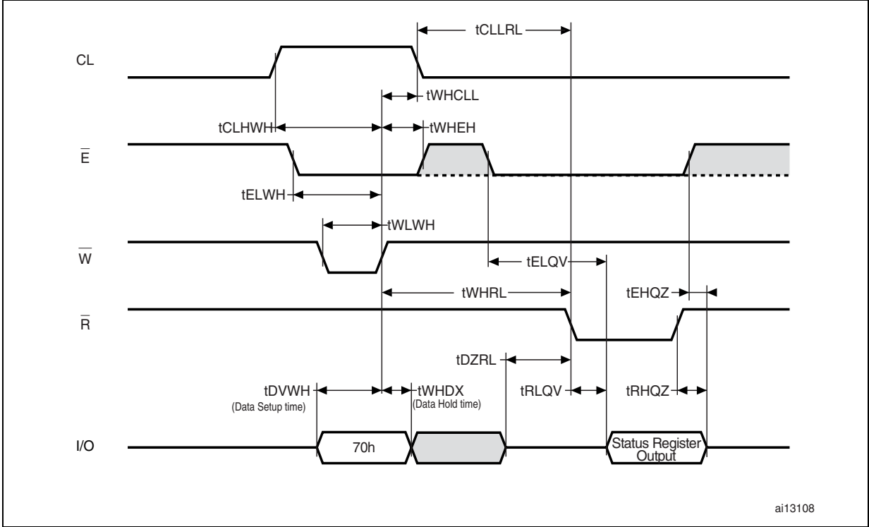
Figure 23. Read Status Register AC Waveform
