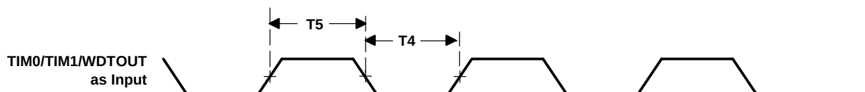
Figure 5–28. TIM0/TIM1/WDTOU Timings When Configured as Timer Input Pins
