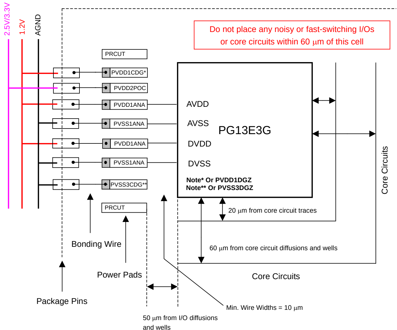
Place & Route Example (with TSMC Universal Std I/O Library)
