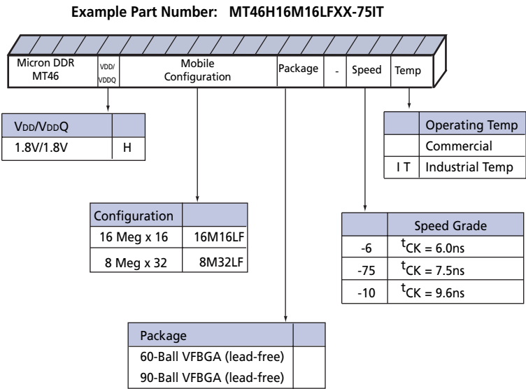
Figure 2: 256Mb Mobile DDR Part Numbering
