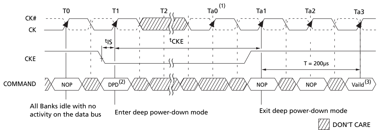
Figure 35: Deep Power-Down
