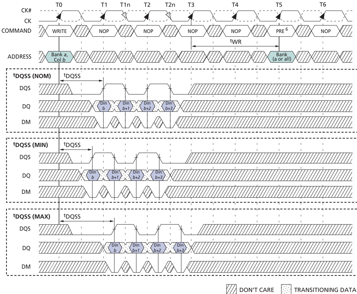
Figure 28: WRITE-to-PRECHARGE – Uninterrupting
