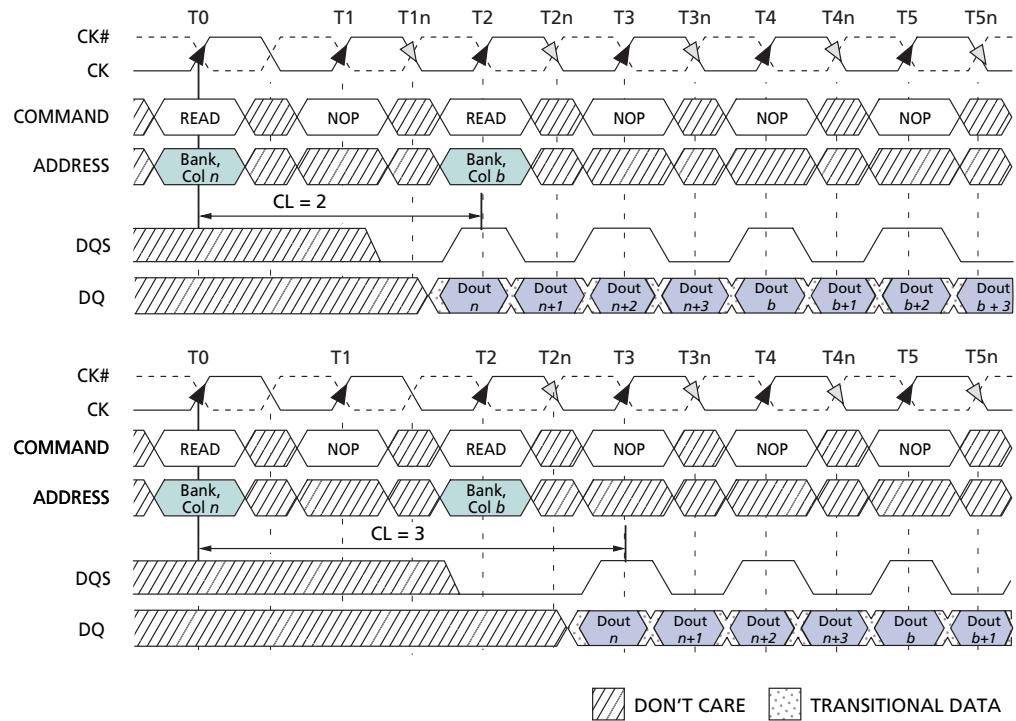
Figure 14: Consecutive READ Burst
