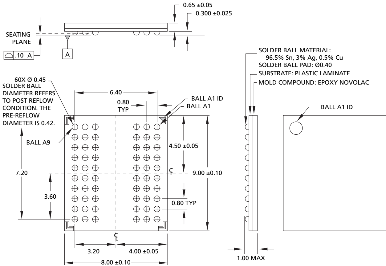
Figure 49: 60-Ball VFBGA Package
