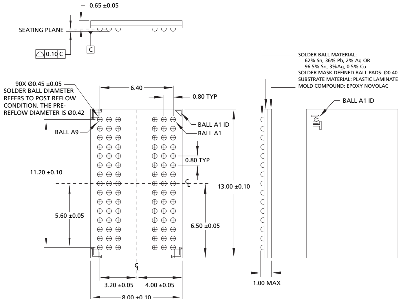
Figure 50: 90-Ball VFBGA Package
