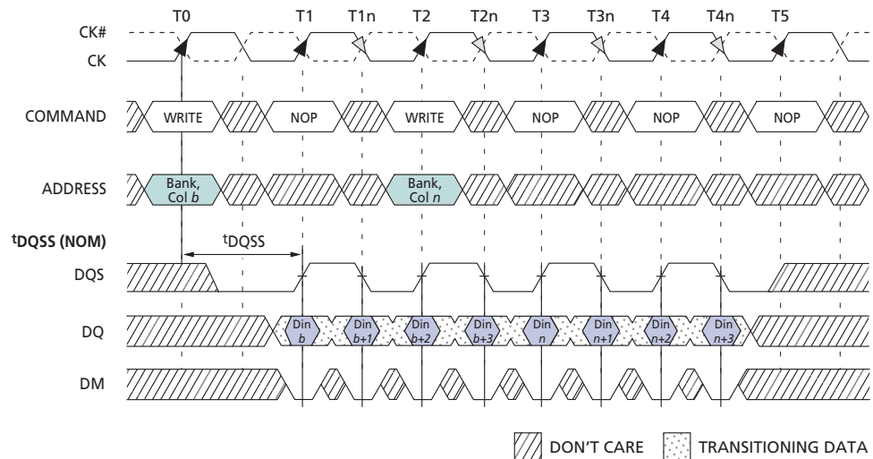
Figure 22: Consecutive WRITE-to-WRITE
