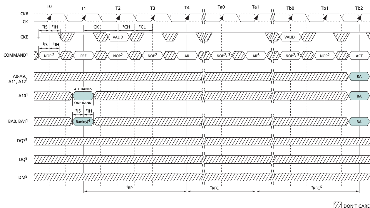
Figure 42: Auto Refresh Mode
