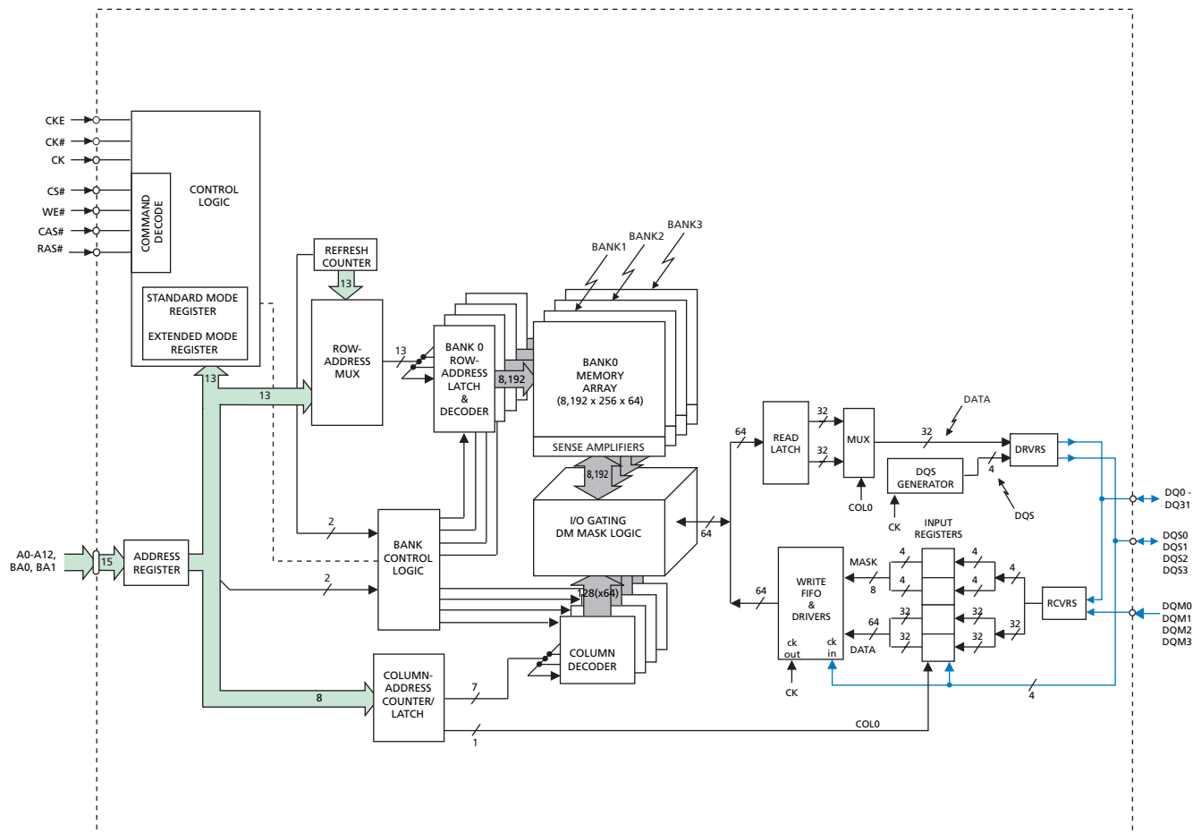
Figure 4: Functional Block Diagram: 8 Meg x 32 Mobile DDR SDRAM
