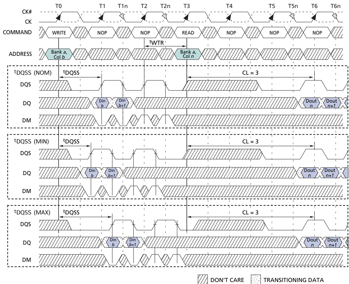
Figure 26: WRITE-to-READ – Interrupting
