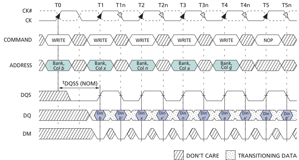
Figure 24: Random WRITE Cycles
