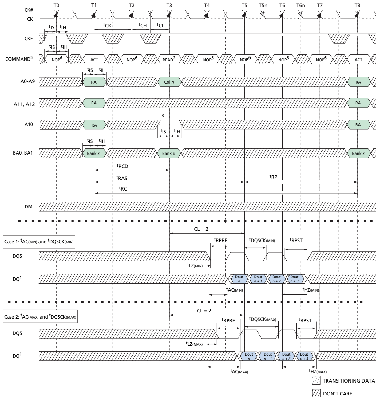
Figure 45: Bank Read – With Auto Precharge
