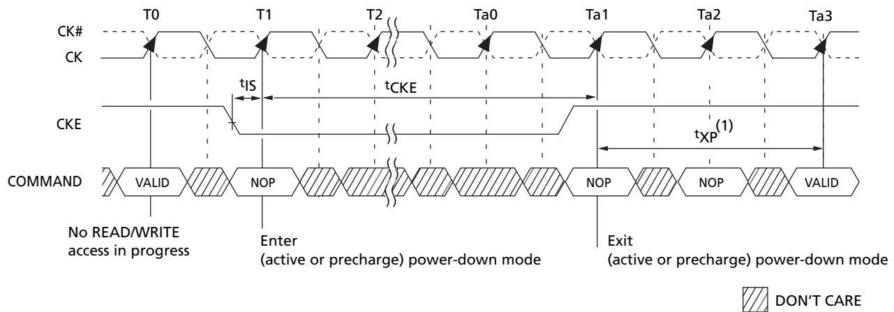
Figure 33: Power-Down in ACTIVE or Precharge Modes
