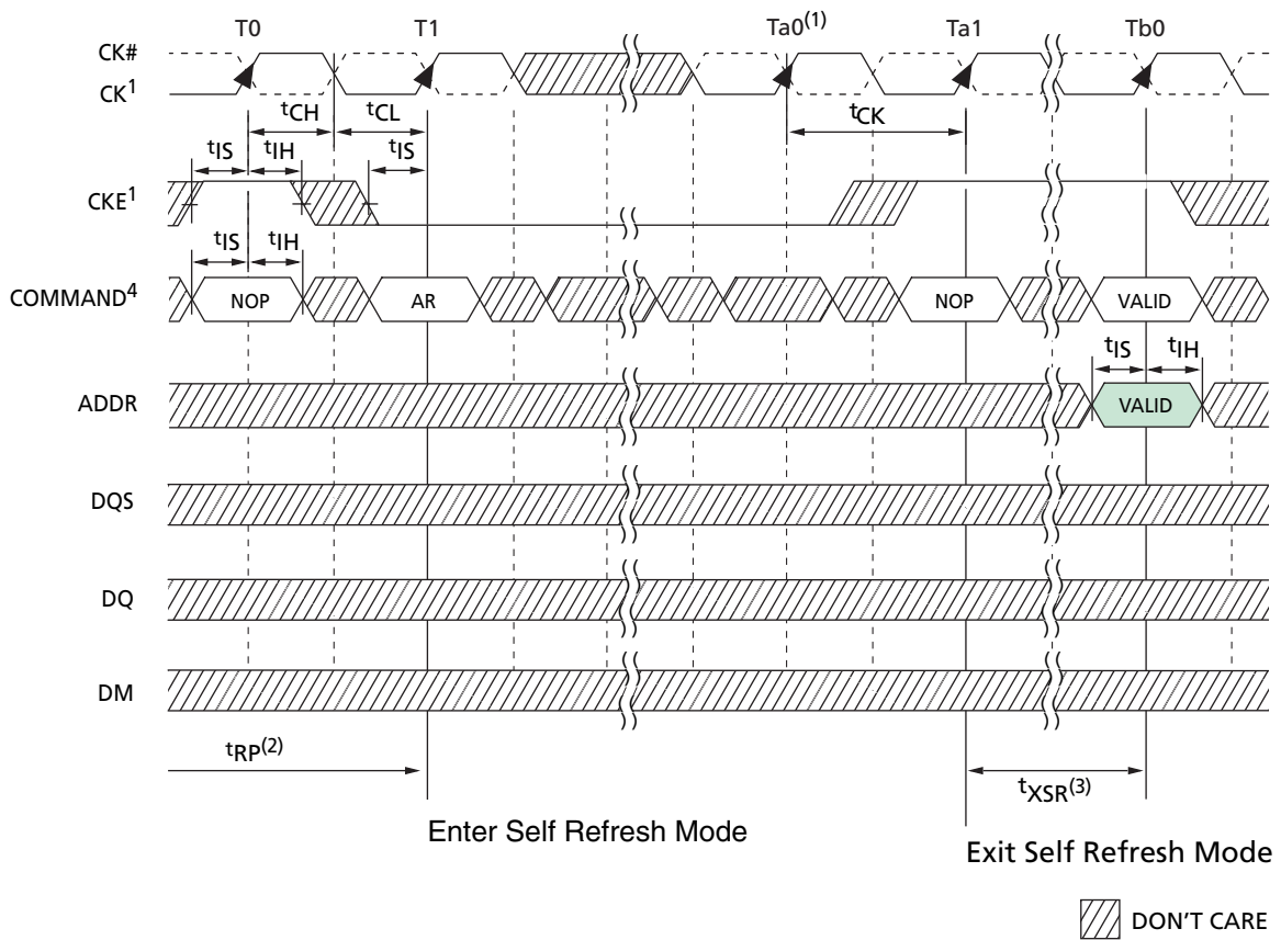
Figure 43: Self Refresh Mode
