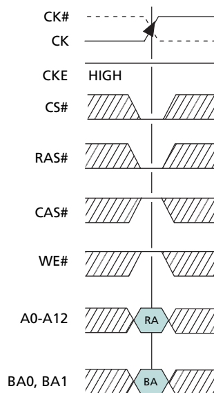
Figure 10: Activating a Specific Row in a Specific Bank
