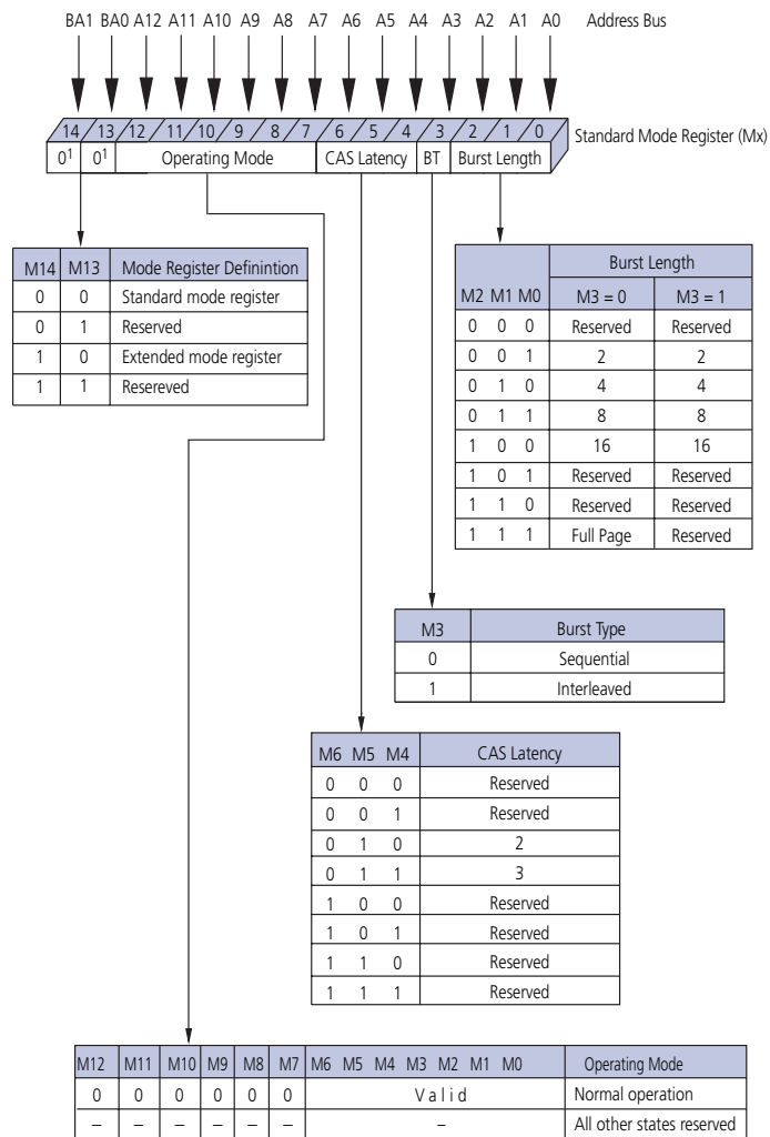
Figure 6: Standard Mode Register Definition
