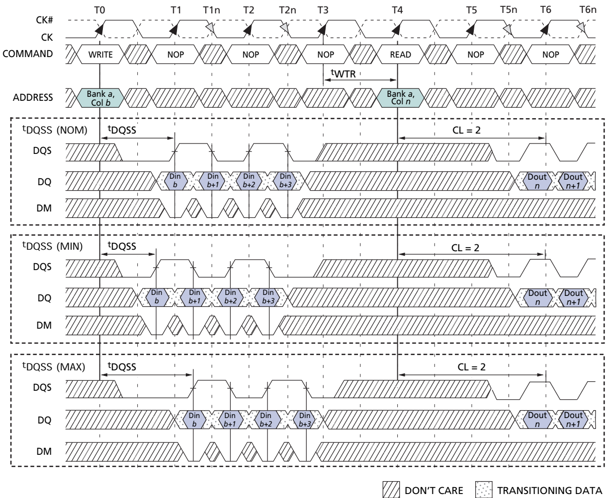
Figure 25: WRITE-to-READ – Uninterrupting
