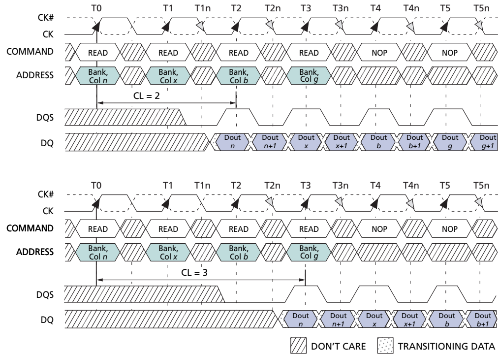
Figure 16: Random READ Accesses
