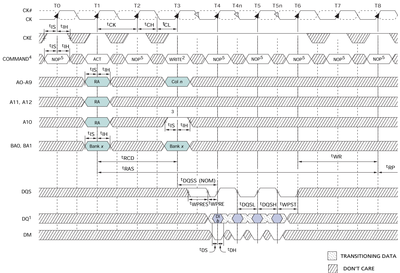
Figure 47: Bank Write – With Auto Precharge
