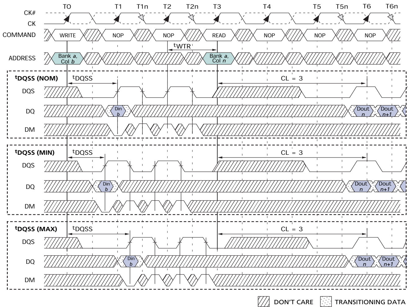
Figure 27: WRITE-to-READ – Odd Number of Data, Interrupting
