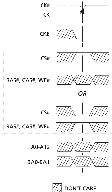
Figure 32: Power-Down Command in ACTIVE or Precharge Modes
