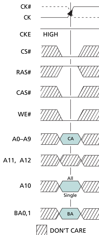
Figure 31: PRECHARGE Command
