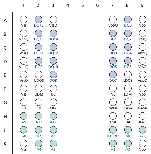
Figure 1: 60-Ball VFBGA
