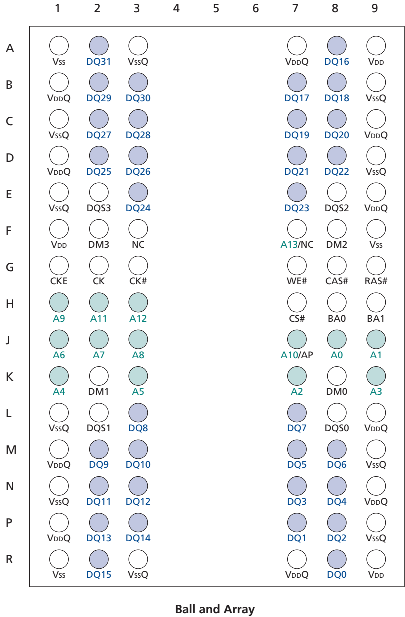
Figure 5: 90-Ball VFBGA (Top View) – 8mm x 13mm
