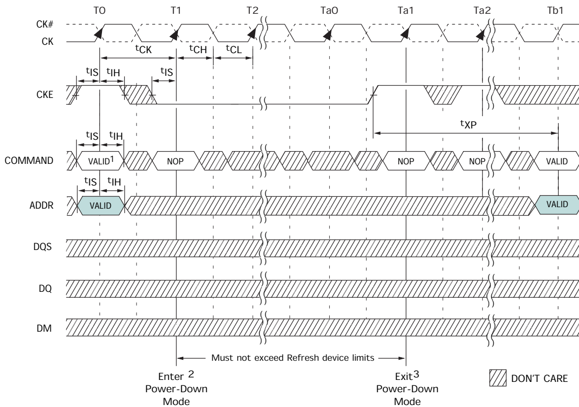
Figure 41: Power Down Mode (Active or Precharge)
