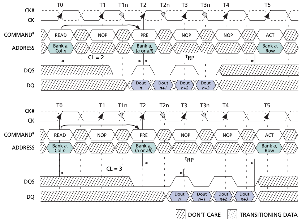
Figure 19: READ-to-PRECHARGE
