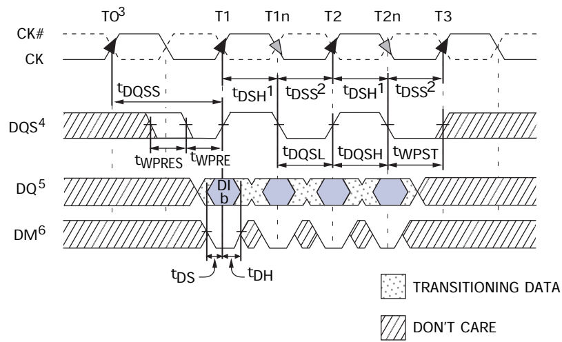
Figure 39: Data Input Timing
