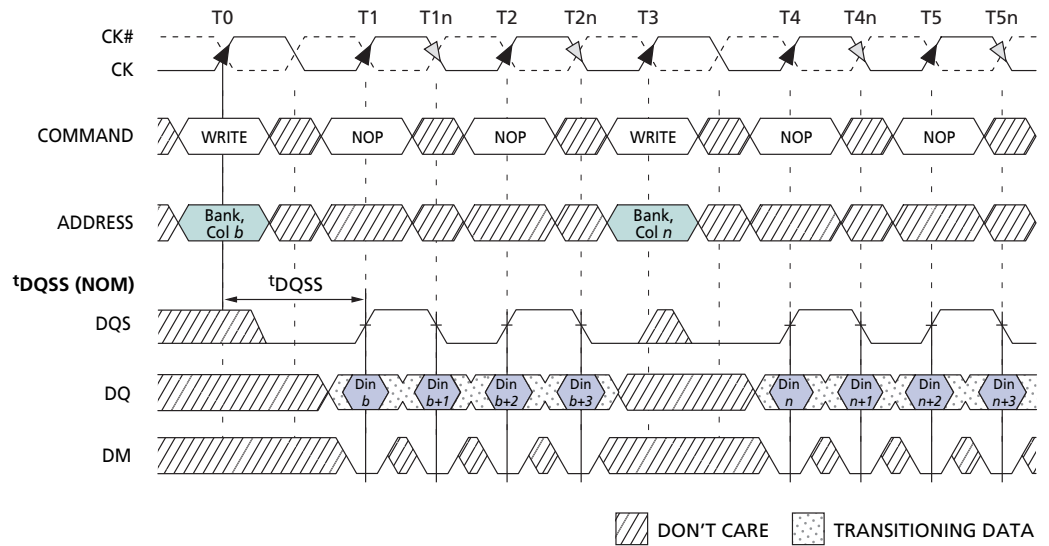
Figure 23: Nonconsecutive WRITE-to-WRITE
