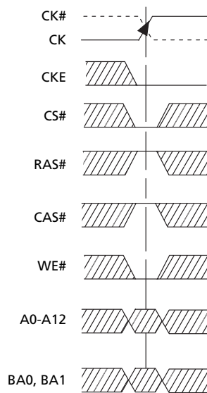
Figure 34: Deep Power-Down Command
