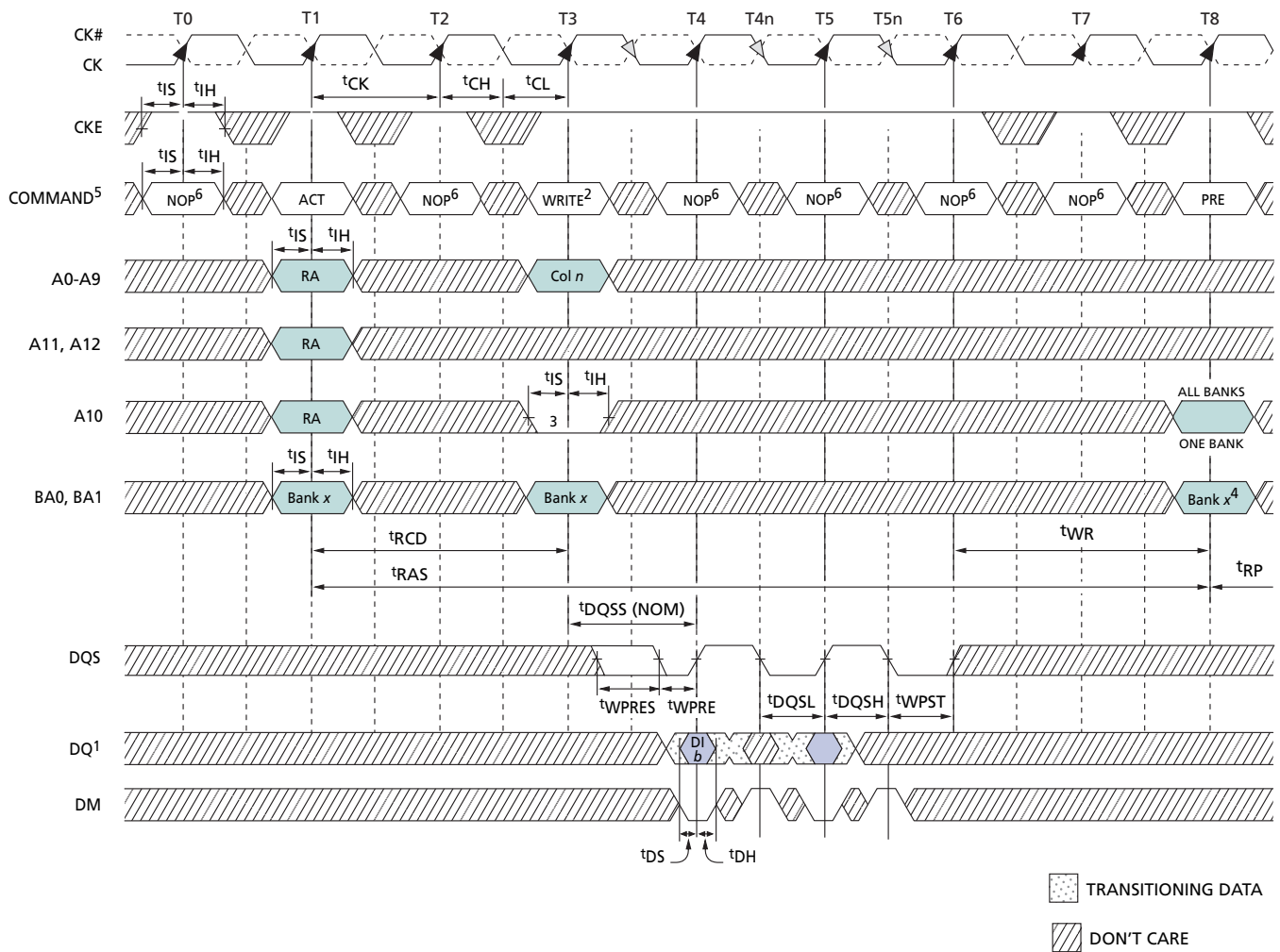
Figure 48: Write – DM Operation
