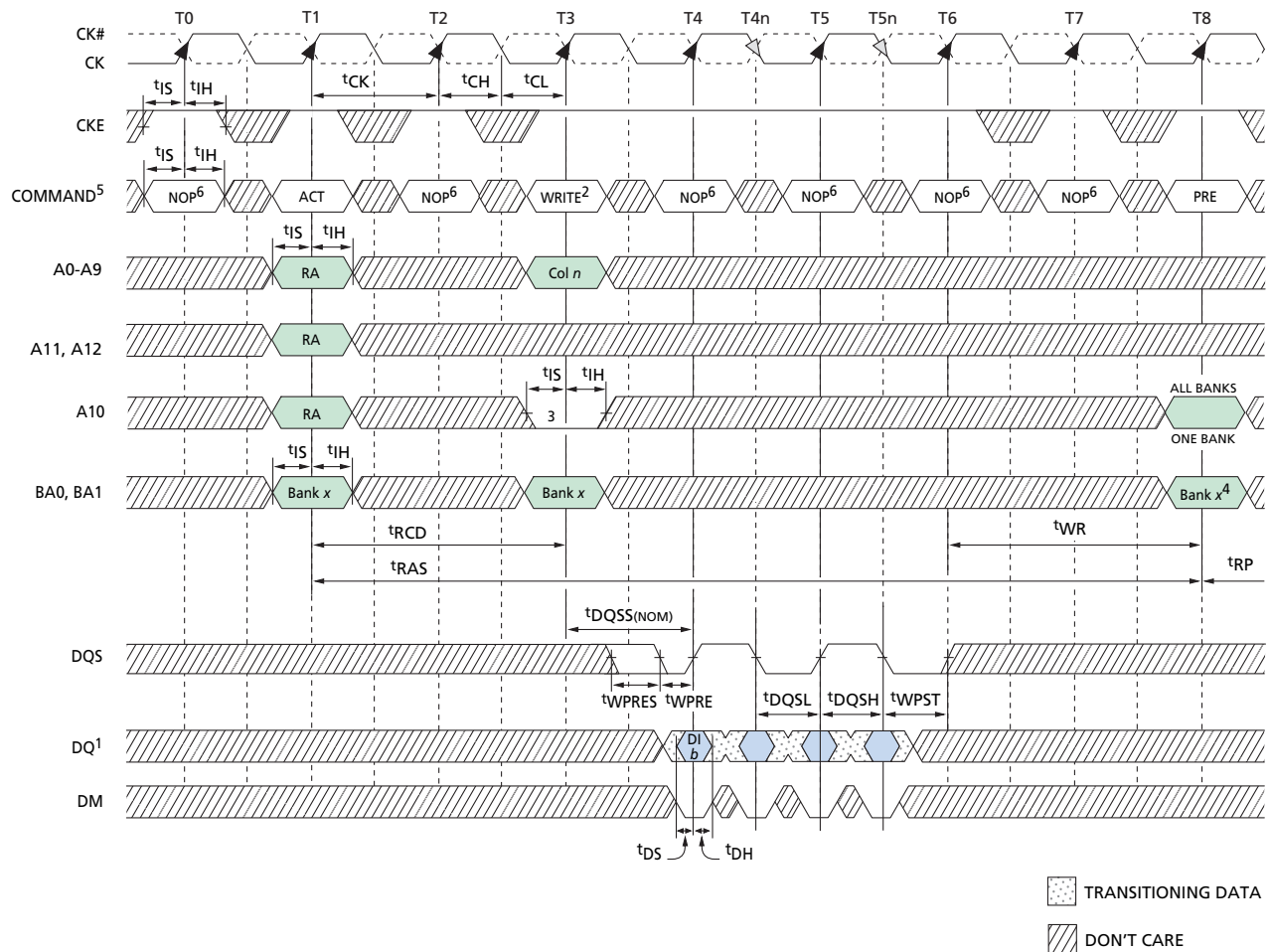
Figure 46: Bank Write – Without Auto Precharge
