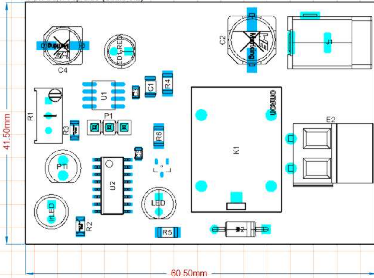
View from Top side (Scale 5:2)
