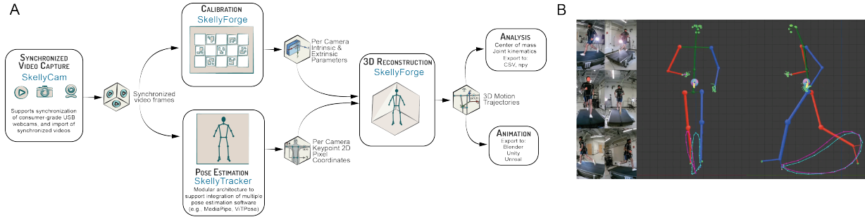
Figure 1: The FreeMoCap workflow and its component repositories (blue). (A) Synchronized video from consumer-grade USB webcams (skellycam) is processed through camera calibration and 3D reconstruction (skellyforge) and modular pose estimation (skellytracker), producing 3D motion trajectories for downstream analysis or animation export. Separation of the pipeline by domain allows individual components to be modified or replaced independently. (B) Reconstructed 3D trajectories alongside the source camera views.
